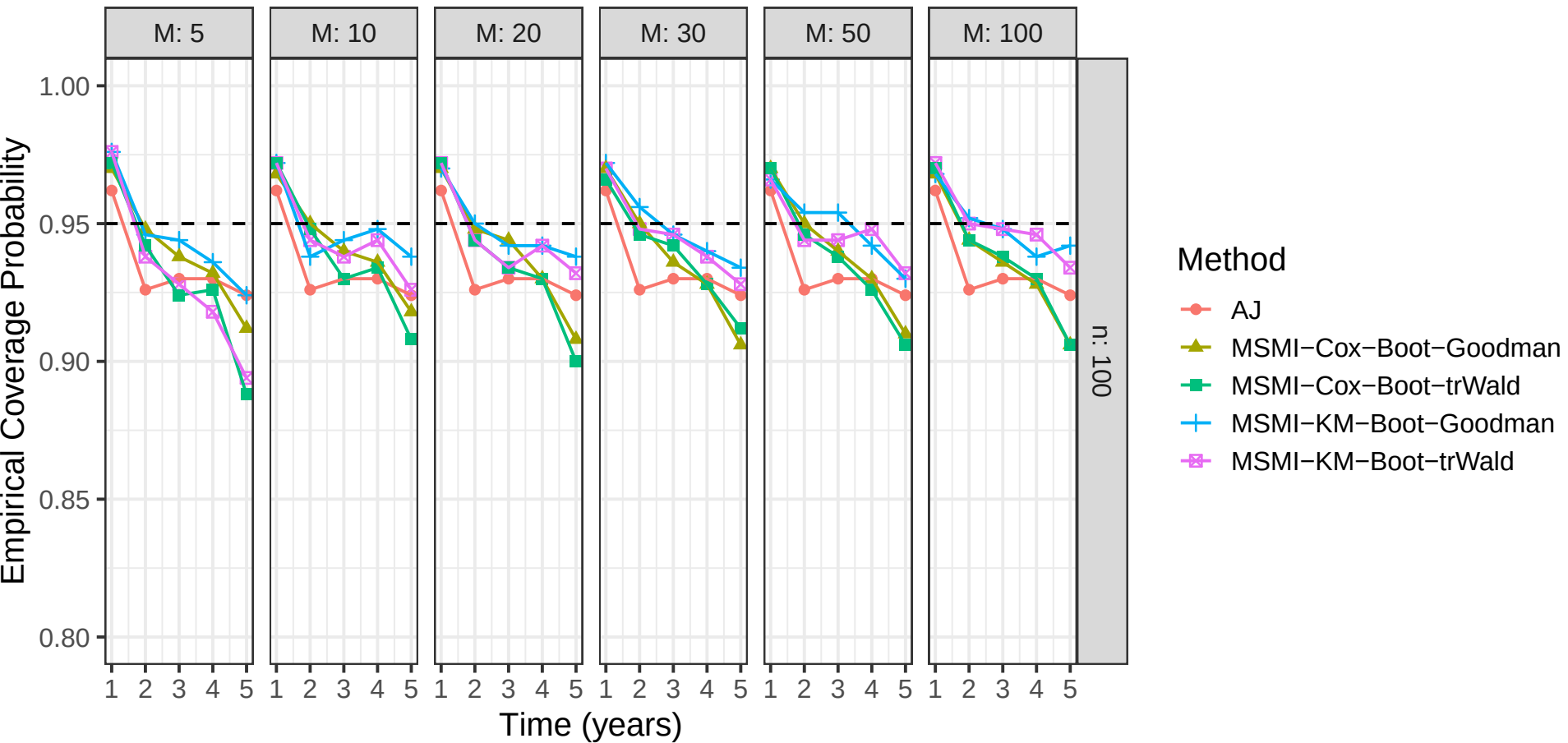
Coverage for LIHC (beta = 0)
