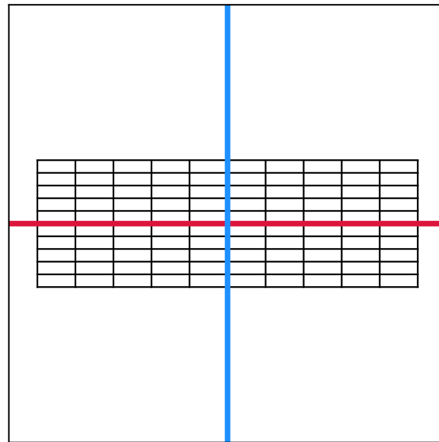
Distinct real eigenvalues (anisotropic scaling)
