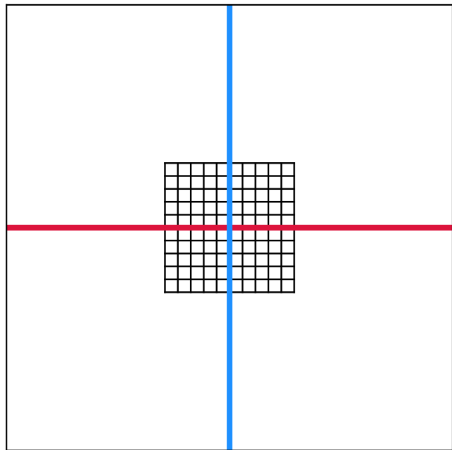
Identity map (no geometric change)
