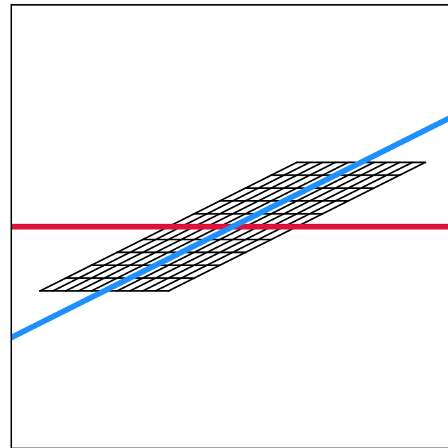
Repeated eigenvalue (shear, one eigendirection)
