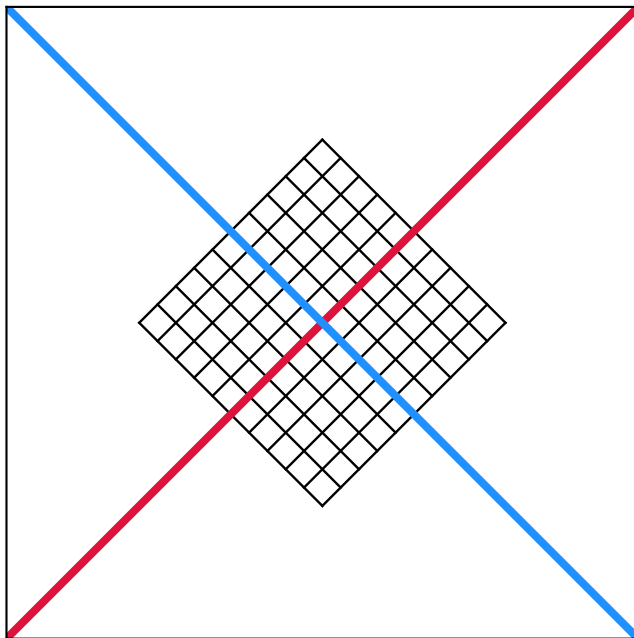
Complex eigenvalues (rotation + scale)
