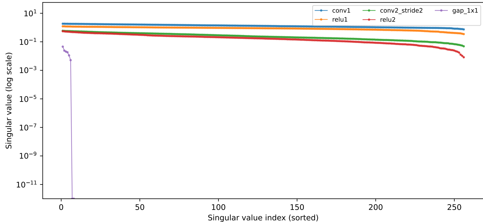
Jacobian singular values across layers (UNTRAINED, same probe image)
