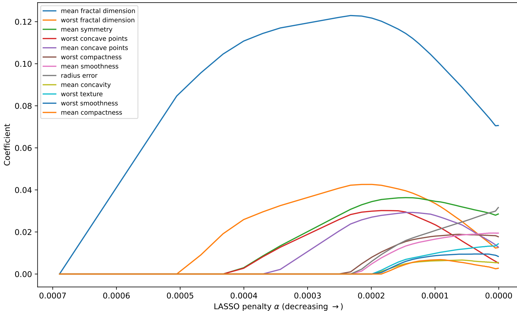
LIME + weighted LASSO path (class 0, center 0)
