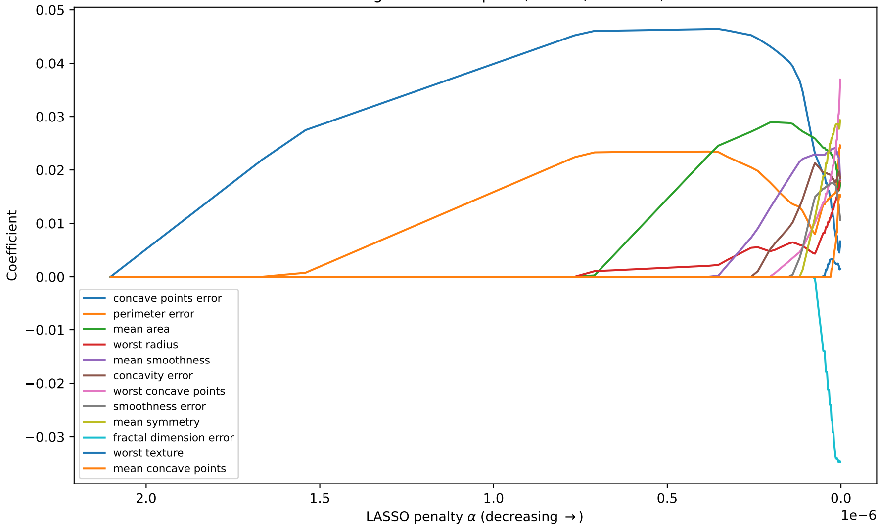
LIME + weighted LASSO path (class 0, center 2)
