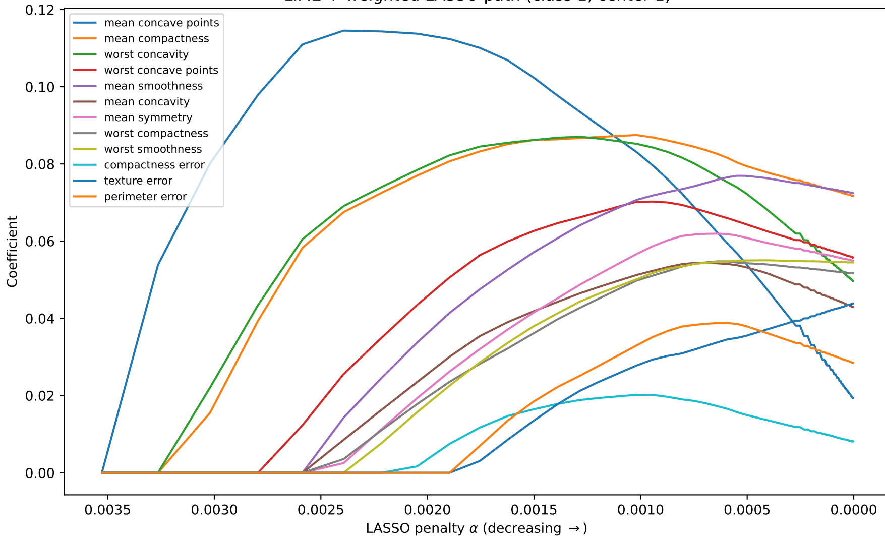
LIME + weighted LASSO path (class 1, center 1)
