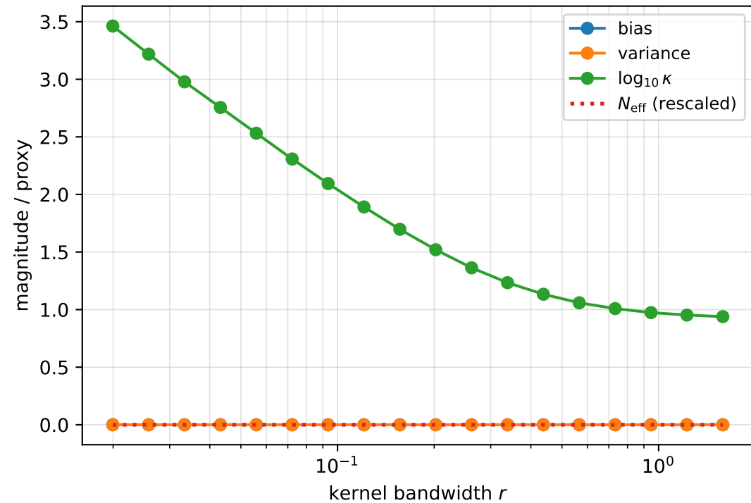
Linear: f(x) = w^\top x
