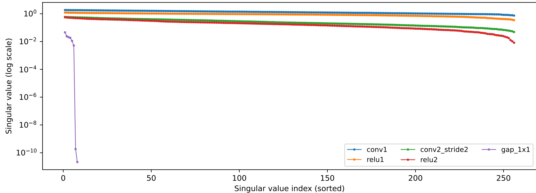
Untrained Jacobian Singular Values Across Layers
