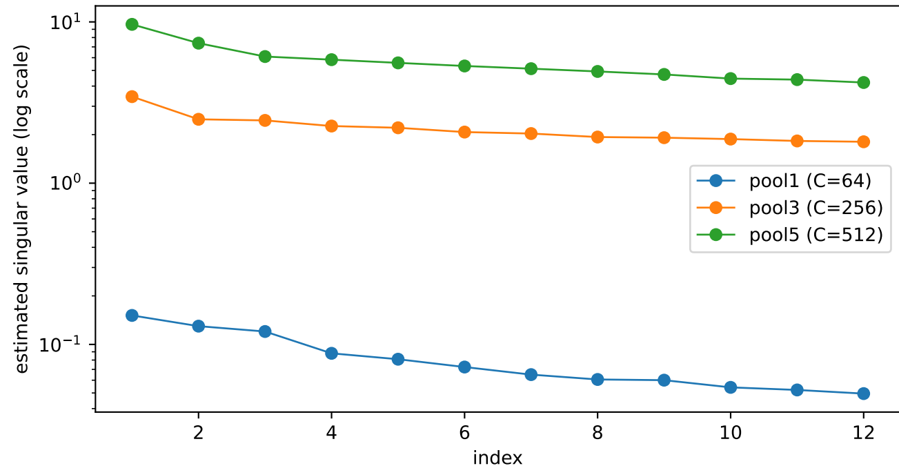
VGG16 (ImageNet) — top singular values of J = dz/dx at different depths
