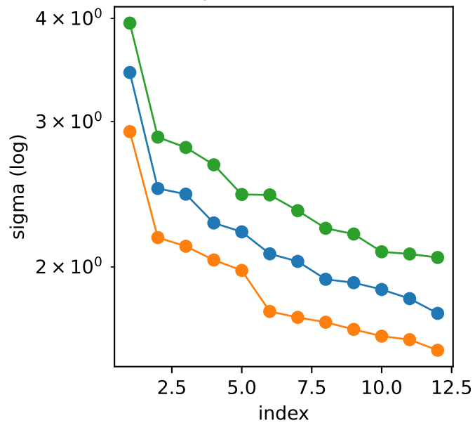
pool3 (C=256)
