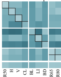
Helmholtz · DeepONet
