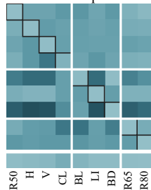
Heat · DeepONet
