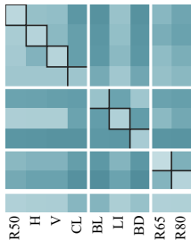
Helmholtz · FNO
