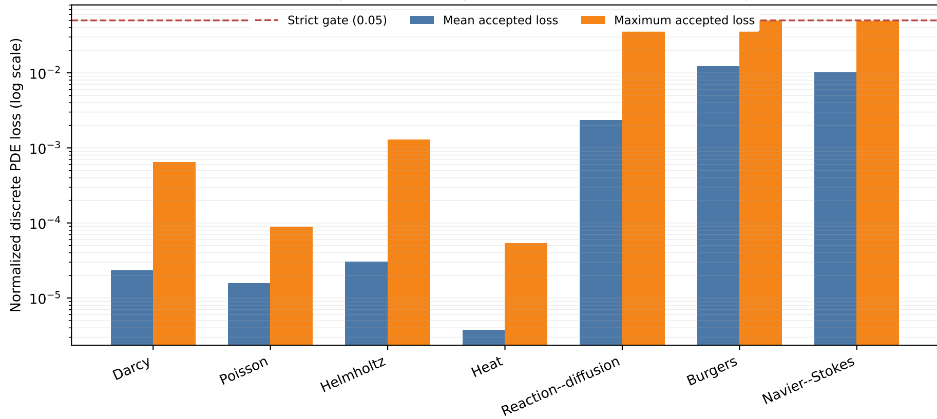
Full-T15 accepted-shard snapshot: 3,348 shards, 557,733 samples
