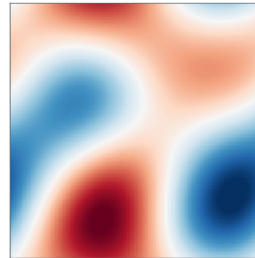
Navier-Stokes
