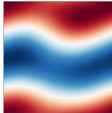
Burgers
