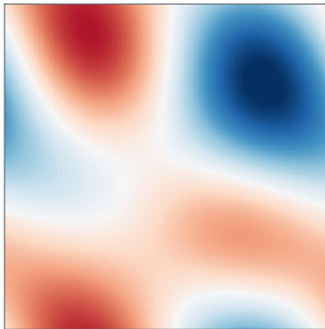
Helmholtz
