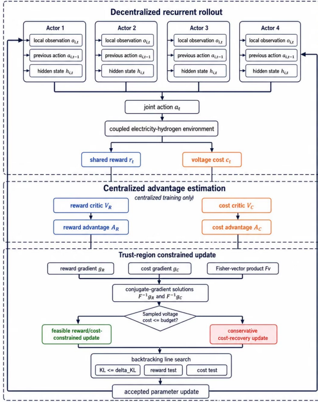
SGR-MACPO training and constrained policy update
