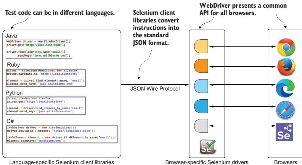
Figure 10.2 Overview of the WebDriver architecture
