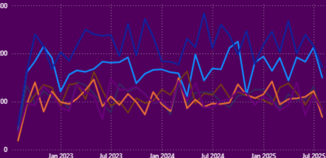
quantity by Year, Month and category
