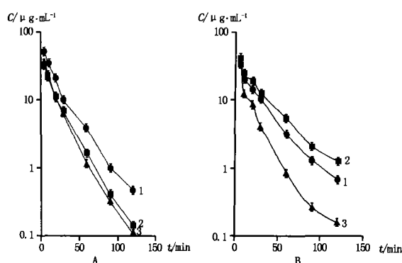
图 2 各组 SD 大鼠静脉注射咪达唑仑后的血浆浓度-时间曲线 Fig 2 Plasma concentration ( \bar{x} \pm SD ) of midazolam after 10 \text{mg} \cdot \text{kg}^{-1} intravenous dose following pretreatment with 100 \text{mg} \cdot \text{kg}^{-1} dexamethasone or 25 \text{mg} \cdot \text{kg}^{-1} zolmitriptan once daily for 3 days in SD-rats A. 雄性大鼠 (male rats) B. 雌性大鼠 (female rats) 1. 空白对照 (control) 2. 佐米曲坦 (zolmitriptan) 3. 地塞米松 (dexamethasone)
