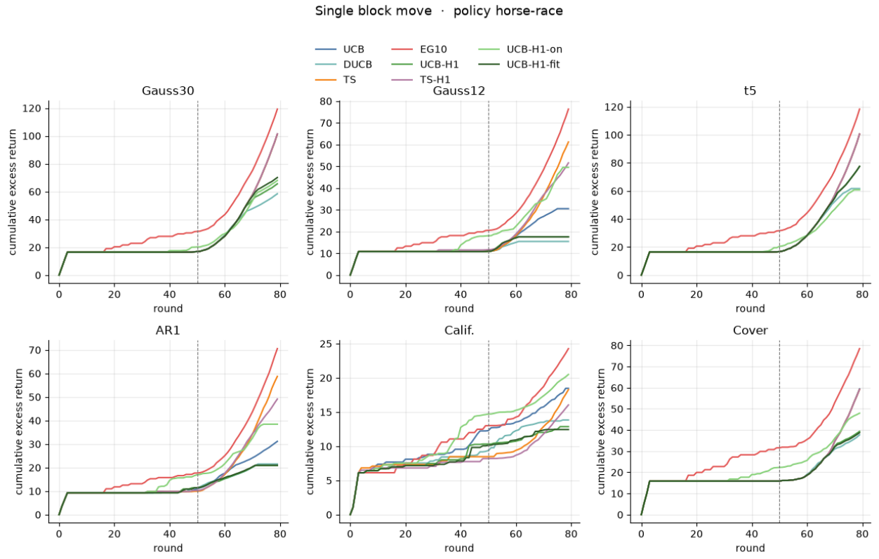
Figure 36: Cumulative excess return, single block move.
