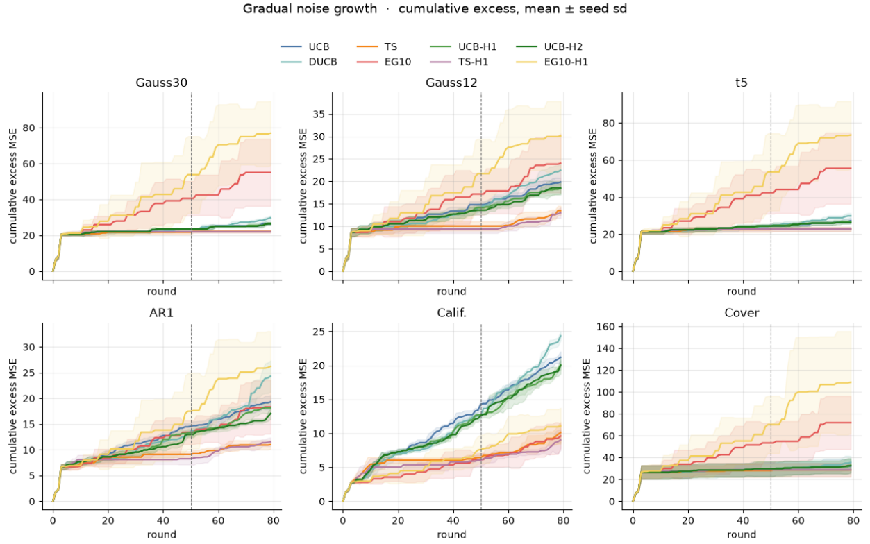
Figure 13: Cumulative excess MSE, gradual noise growth. Mean across four seeds, band is the seed standard deviation. The dashed line is the first round with mixing weight at least 1/2 .
