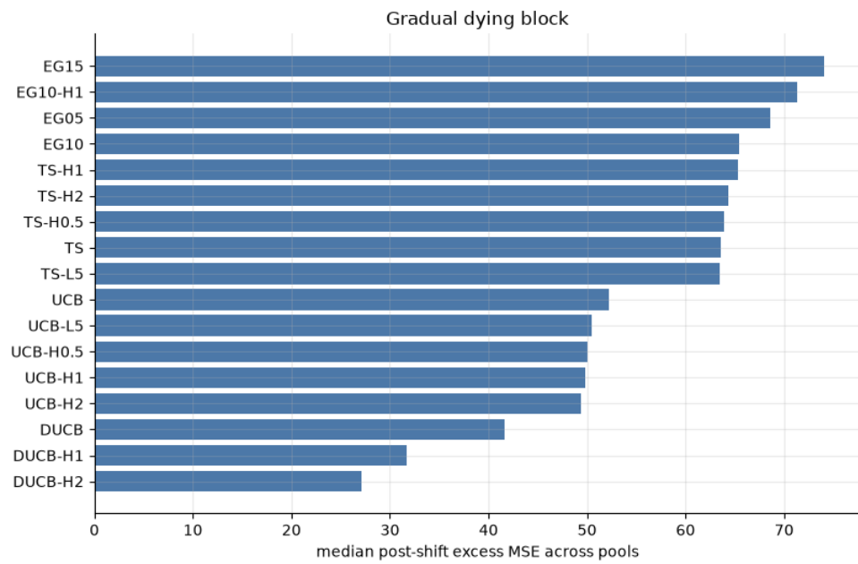
Figure 29: Median post-shift excess across the six pools, gradual dying block. Lower is better.
