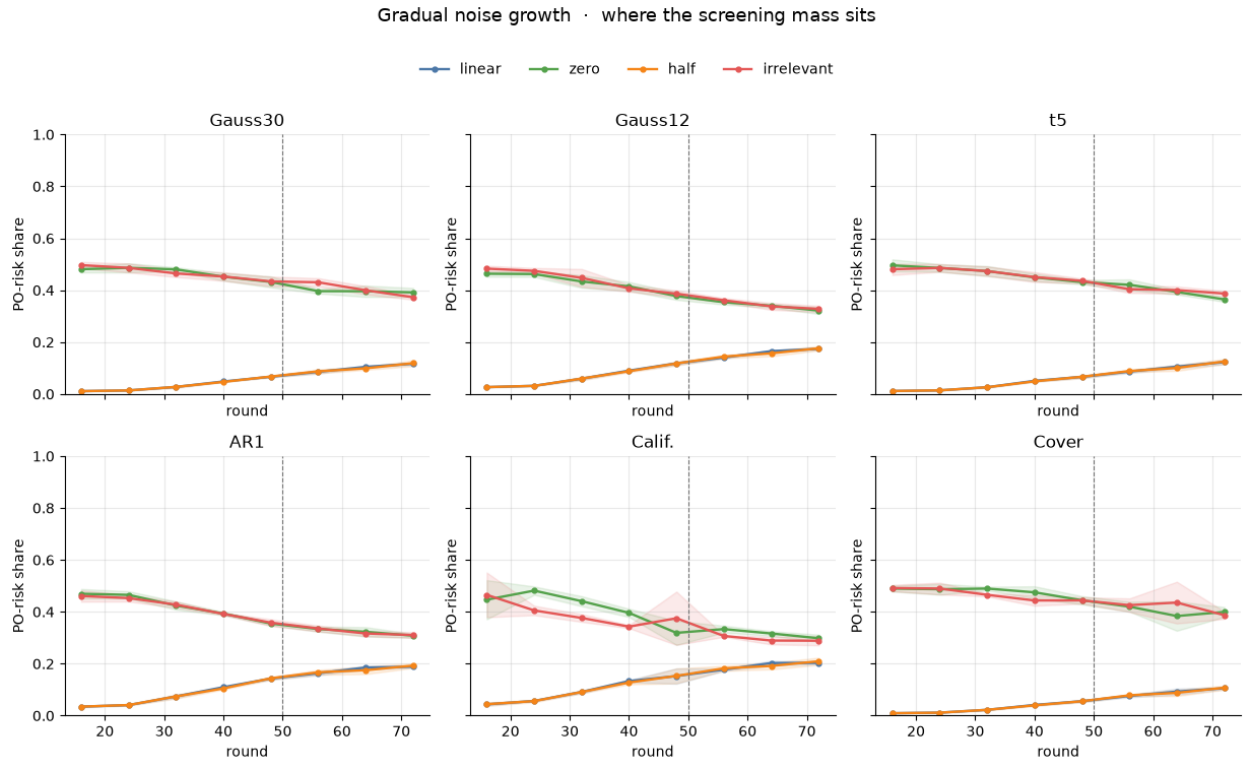
Figure 23: PO-risk shares, gradual noise growth. Mean across four seeds.
