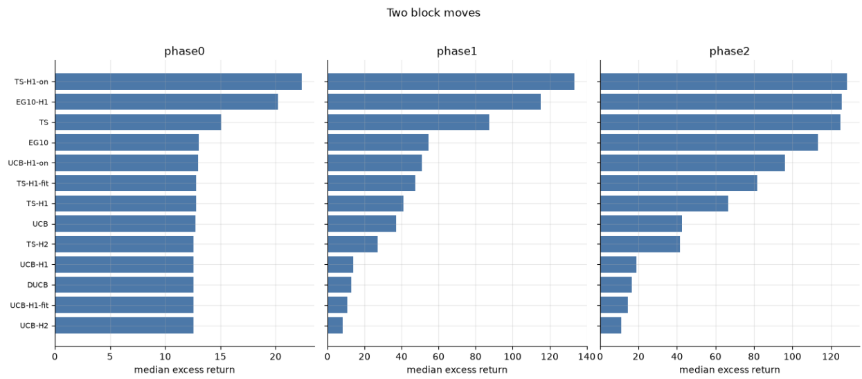
Figure 39: Median excess return, two block moves.
