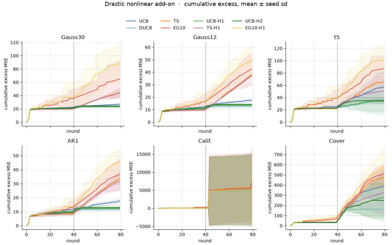
Figure 12: Cumulative excess MSE, drastic nonlinear add-on. Mean across four seeds, band is the seed standard deviation. The dashed line is the first round with mixing weight at least 1/2 .
