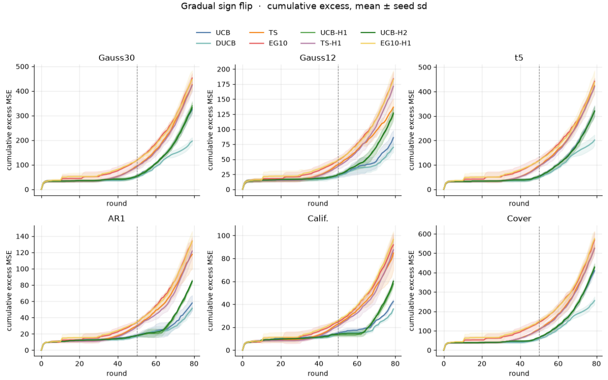
Figure 7: Cumulative excess MSE, gradual sign flip. Mean across four seeds, band is the seed standard deviation. The dashed line is the first round with mixing weight at least 1/2 .
