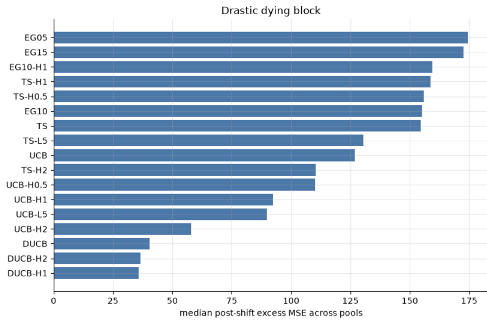
Figure 30: Median post-shift excess across the six pools, drastic dying block. Lower is better.
