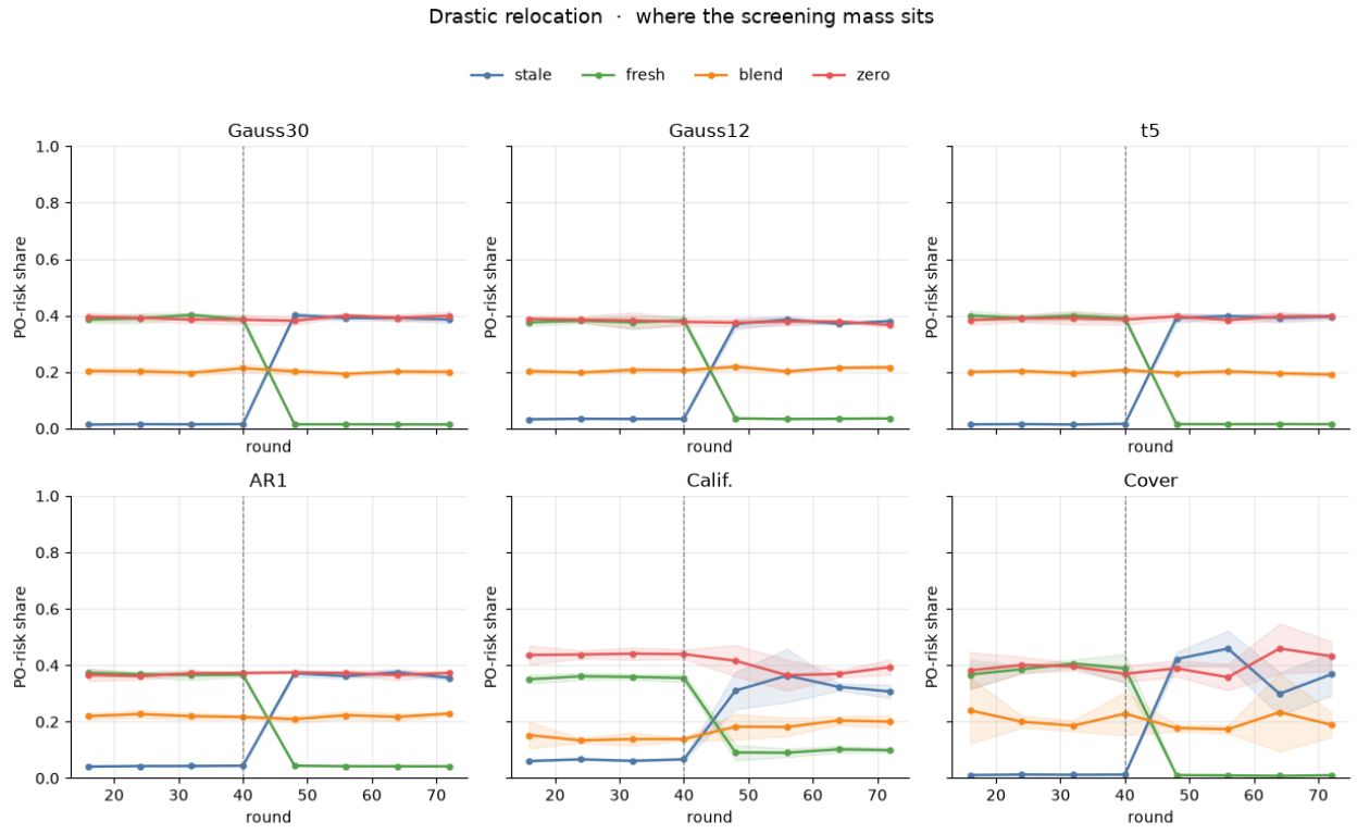
Figure 16: PO-risk shares, drastic relocation. Mean across four seeds.
