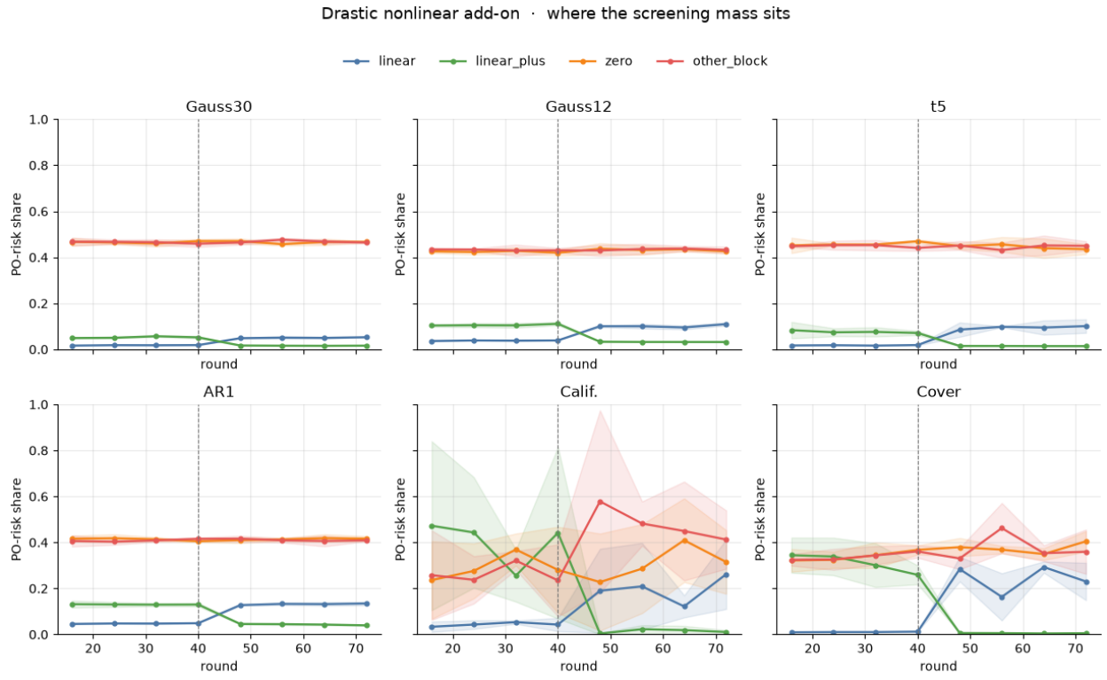
Figure 22: PO-risk shares, drastic nonlinear add-on. Mean across four seeds.
