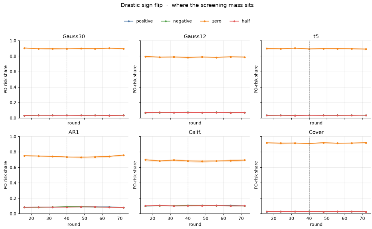
Figure 18: PO-risk shares, drastic sign flip. Mean across four seeds.
