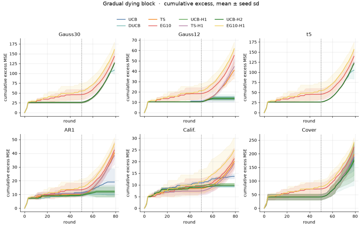
Figure 9: Cumulative excess MSE, gradual dying block. Mean across four seeds, band is the seed standard deviation. The dashed line is the first round with mixing weight at least 1/2 .
