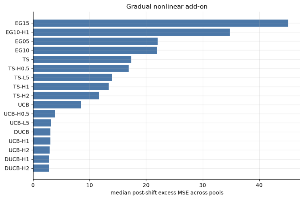
Figure 31: Median post-shift excess across the six pools, gradual nonlinear add-on. Lower is better.
