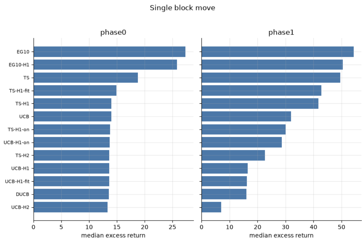
Figure 38: Median excess return, single block move.
