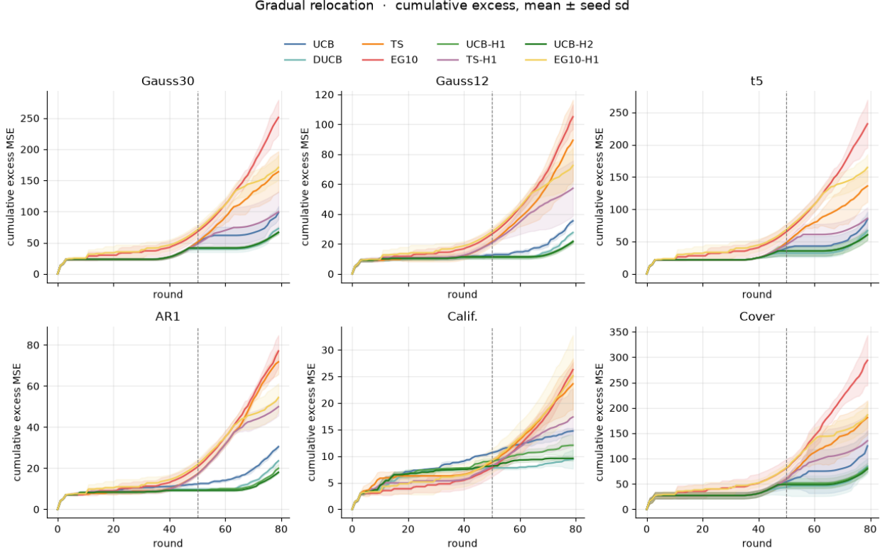
Figure 2: Cumulative excess on a gradual relocation. UCB with \eta = 1 or 2 stays flat after the dashed line. Epsilon-greedy at 10%, with or without the tax, keeps accumulating. Thompson sampling without the tax tracks the exploring rules; with \eta = 1 it moves toward UCB.
