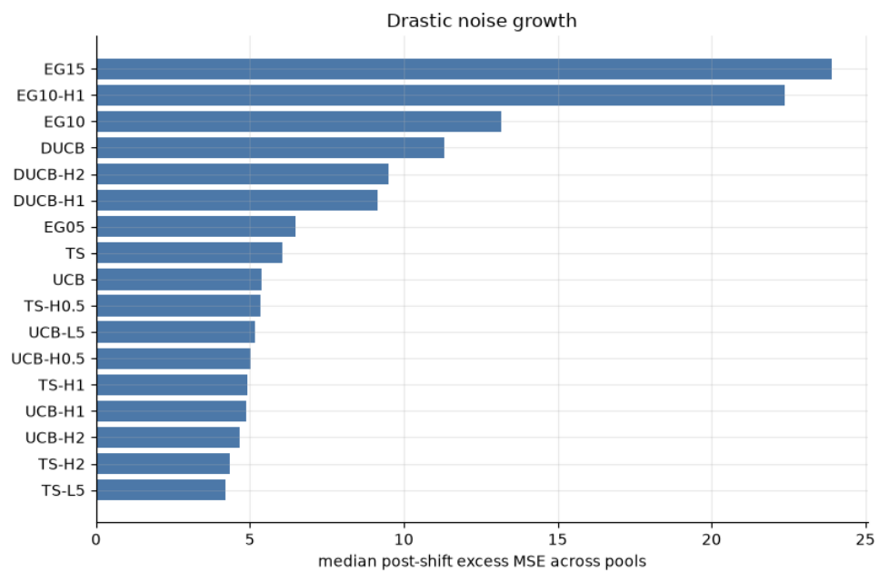
Figure 34: Median post-shift excess across the six pools, drastic noise growth. Lower is better.
