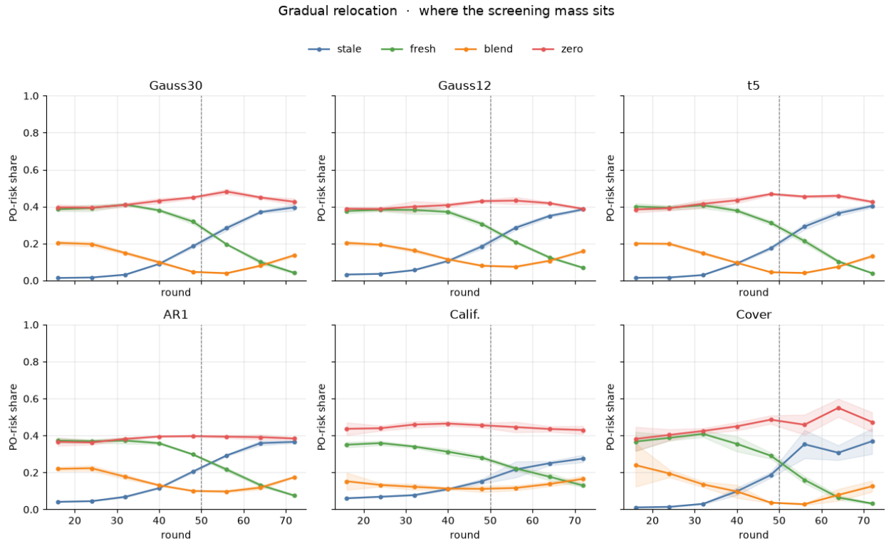
Figure 15: PO-risk shares, gradual relocation. Mean across four seeds.
