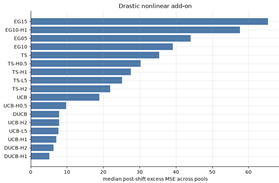
Figure 32: Median post-shift excess across the six pools, drastic nonlinear add-on. Lower is better.
