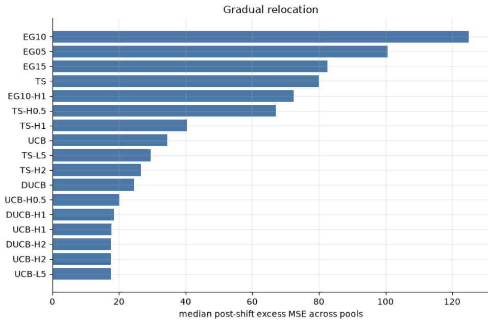
Figure 25: Median post-shift excess across the six pools, gradual relocation. Lower is better.
