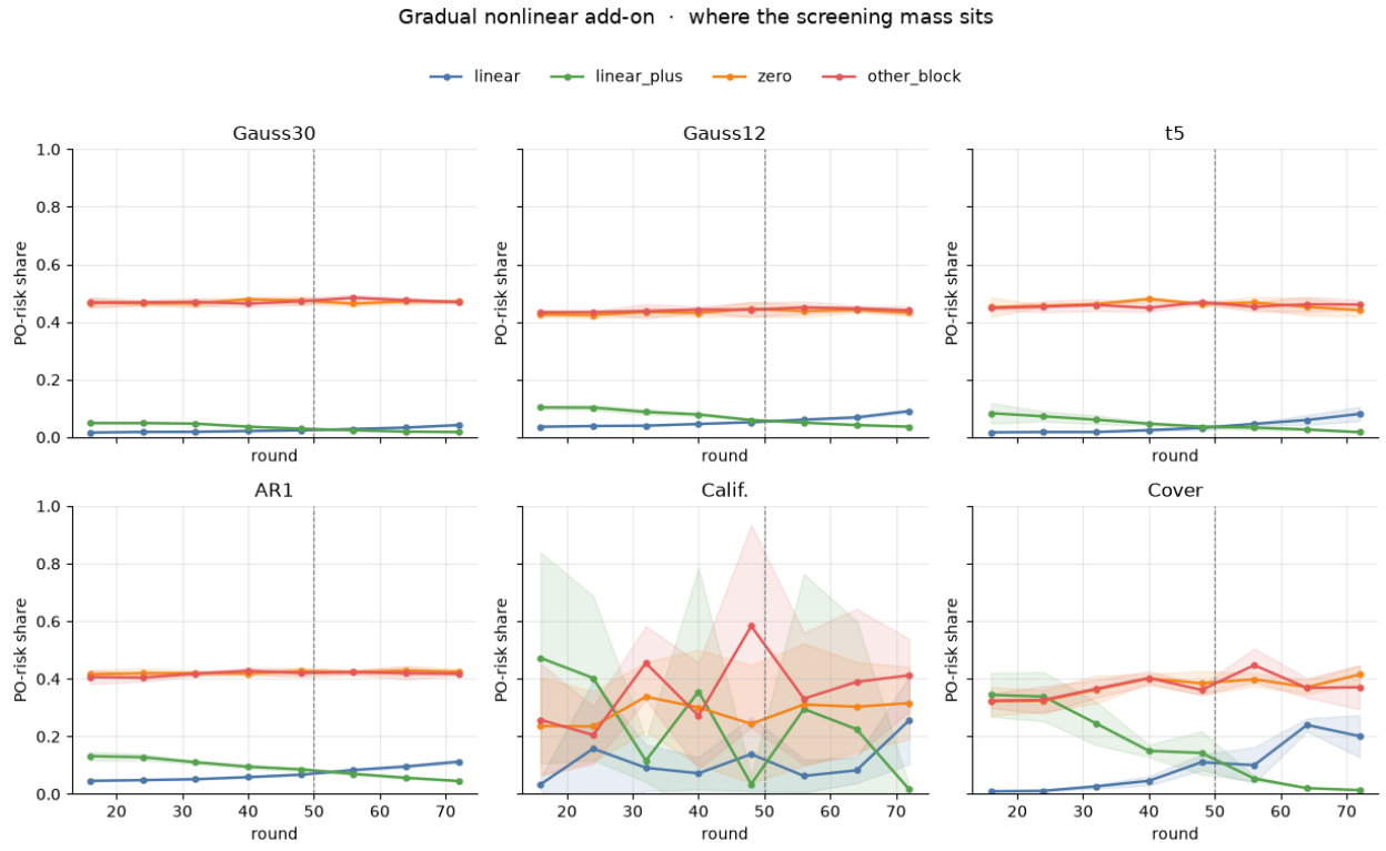
Figure 21: PO-risk shares, gradual nonlinear add-on. Mean across four seeds.
