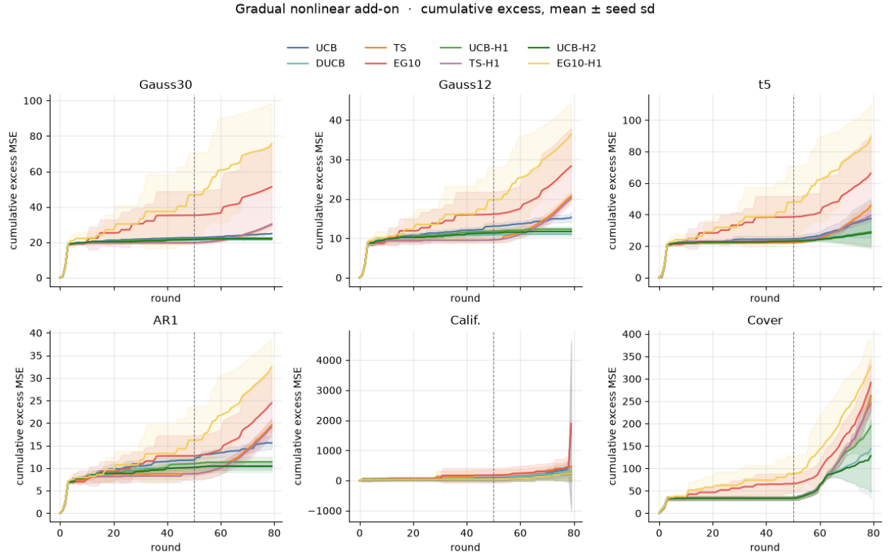
Figure 11: Cumulative excess MSE, gradual nonlinear add-on. Mean across four seeds, band is the seed standard deviation. The dashed line is the first round with mixing weight at least 1/2 .
