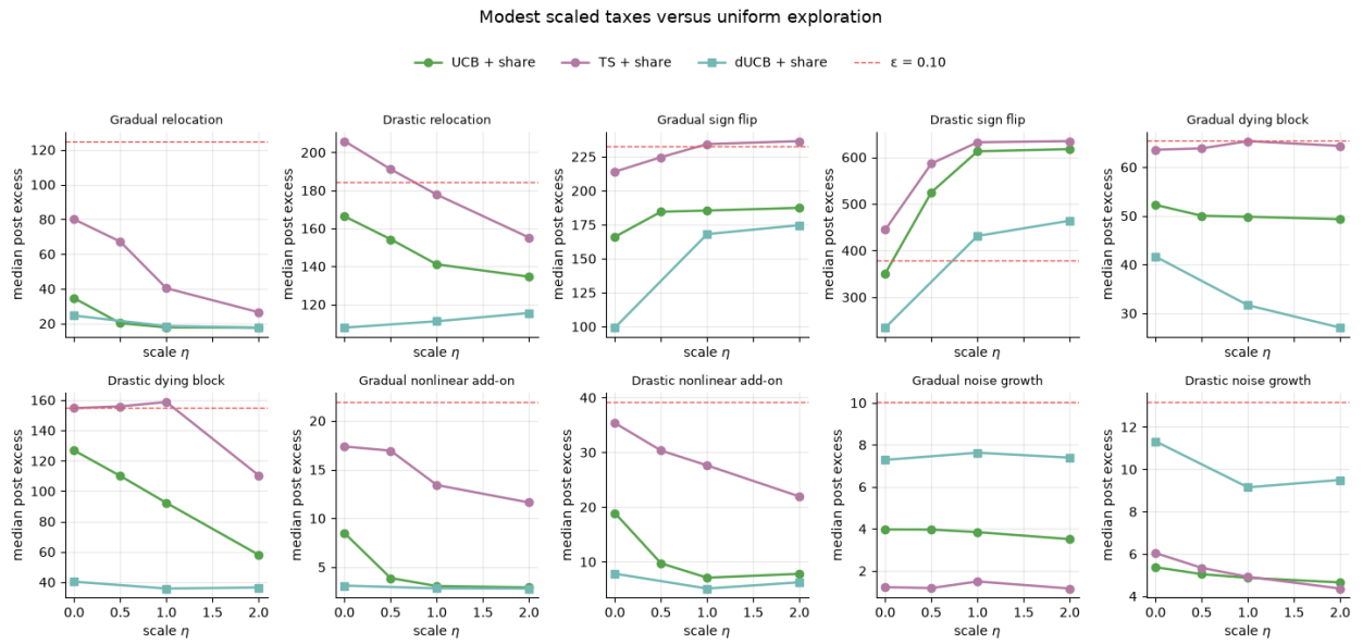
Figure 35: Post-shift excess against \eta , median across pools.
