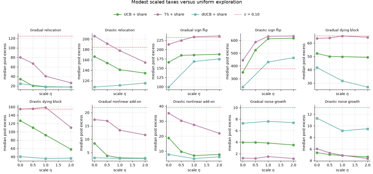
Figure 3: Median post-shift excess against the scale \eta . The dashed line is epsilon-greedy at 10%. Relocation, a dying block, and a nonlinear add-on slope down for UCB. A sign flip slopes up: the tax is the wrong sensor there. Noise growth is already small for Thompson sampling, and discounting sits above UCB because the best card never changes.
