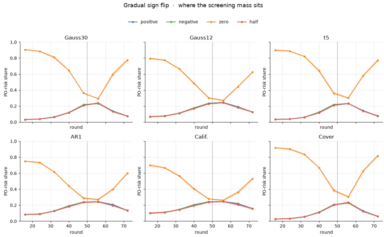
Figure 17: PO-risk shares, gradual sign flip. Mean across four seeds.
