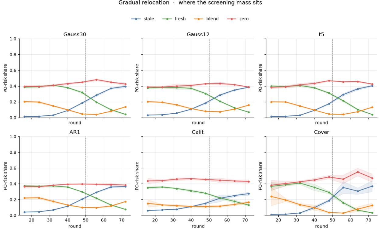
Figure 1: PO-risk shares on a gradual relocation. Before the ramp, the fresh block and the zero score hold the mass, and the stale block, which still carries the signal, sits near zero. After the mixing weight passes 1/2 (dashed line), the fresh share falls and the stale share rises to meet the zero score. The same crossing appears on all six pools. California, with only eight columns, separates more slowly.
