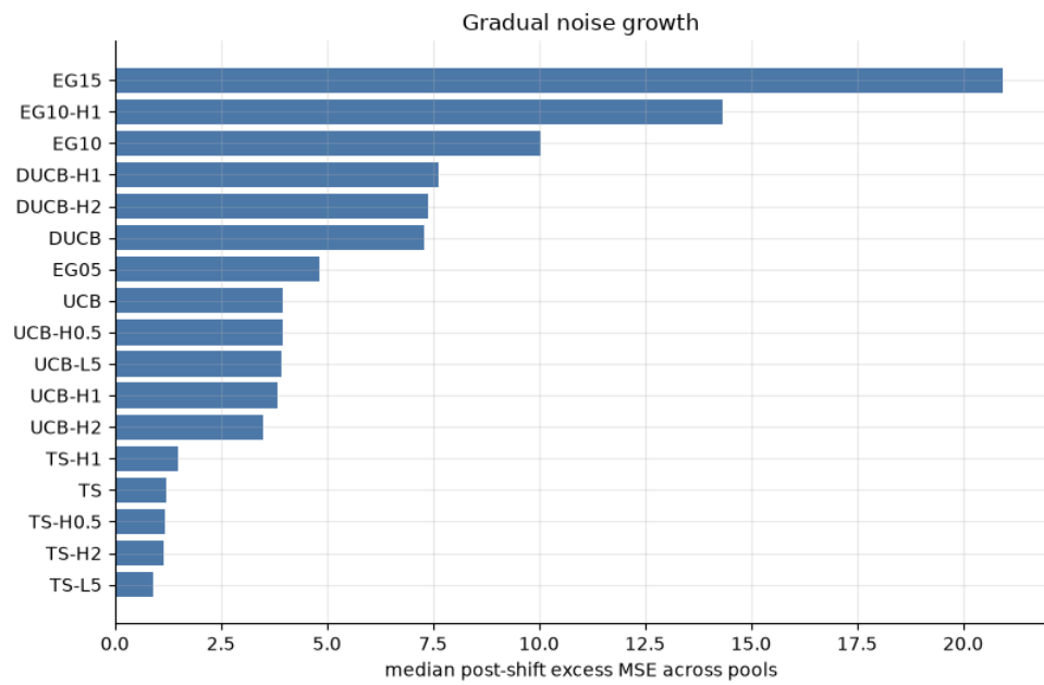
Figure 33: Median post-shift excess across the six pools, gradual noise growth. Lower is better.
