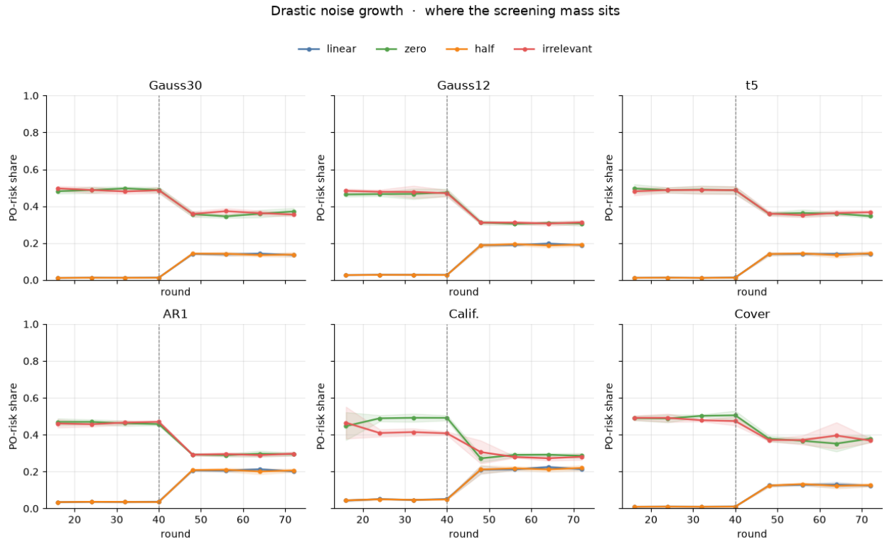
Figure 24: PO-risk shares, drastic noise growth. Mean across four seeds.
