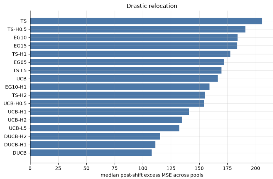
Figure 26: Median post-shift excess across the six pools, drastic relocation. Lower is better.
