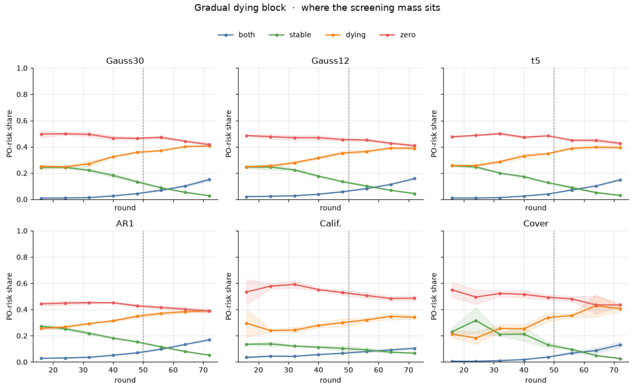
Figure 19: PO-risk shares, gradual dying block. Mean across four seeds.
