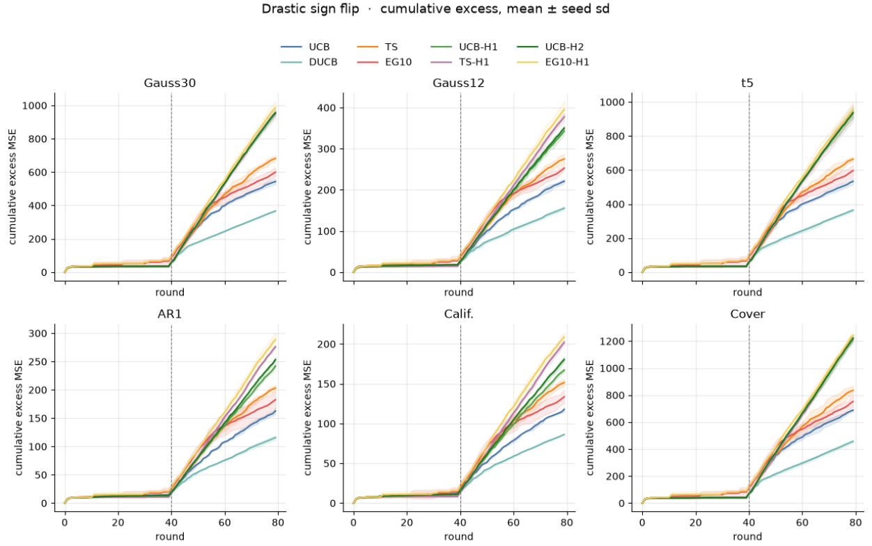
Figure 8: Cumulative excess MSE, drastic sign flip. Mean across four seeds, band is the seed standard deviation. The dashed line is the first round with mixing weight at least 1/2 .
