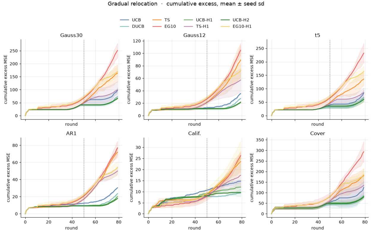
Figure 5: Cumulative excess MSE, gradual relocation. Mean across four seeds, band is the seed standard deviation. The dashed line is the first round with mixing weight at least 1/2 .
