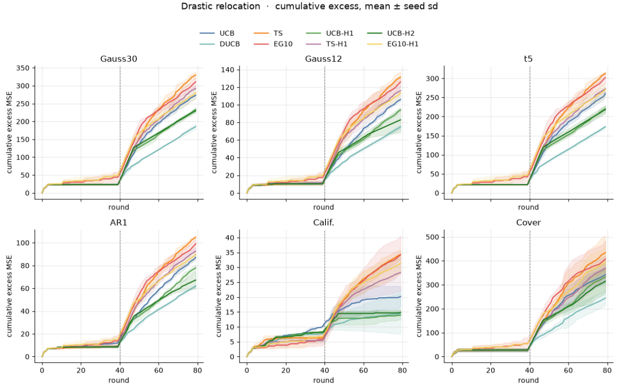
Figure 6: Cumulative excess MSE, drastic relocation. Mean across four seeds, band is the seed standard deviation. The dashed line is the first round with mixing weight at least 1/2 .
