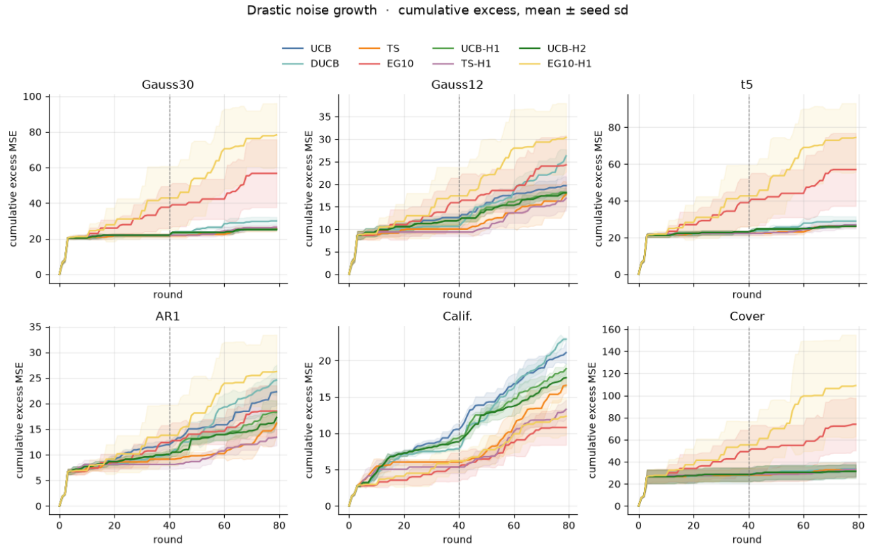
Figure 14: Cumulative excess MSE, drastic noise growth. Mean across four seeds, band is the seed standard deviation. The dashed line is the first round with mixing weight at least 1/2 .
