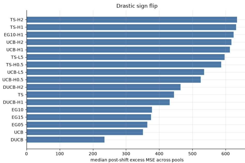
Figure 28: Median post-shift excess across the six pools, drastic sign flip. Lower is better.
