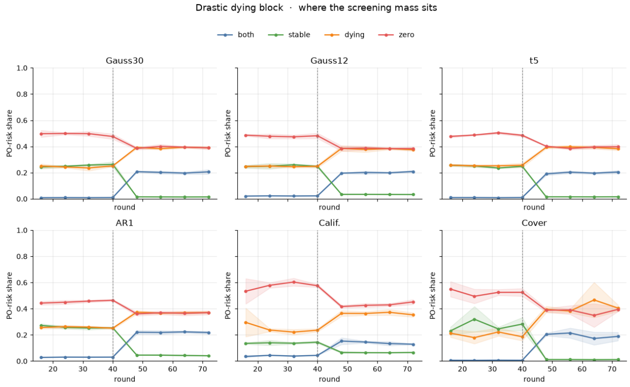
Figure 20: PO-risk shares, drastic dying block. Mean across four seeds.
