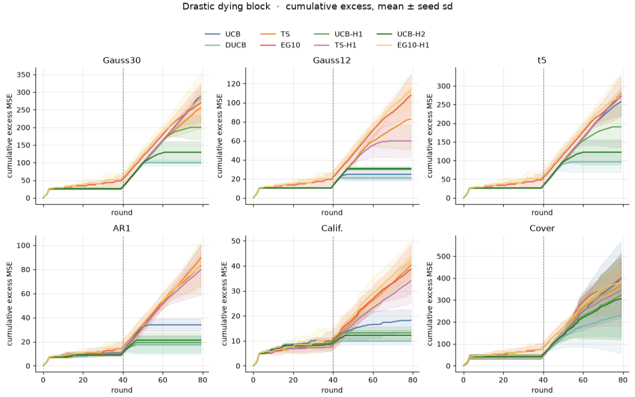
Figure 10: Cumulative excess MSE, drastic dying block. Mean across four seeds, band is the seed standard deviation. The dashed line is the first round with mixing weight at least 1/2 .
