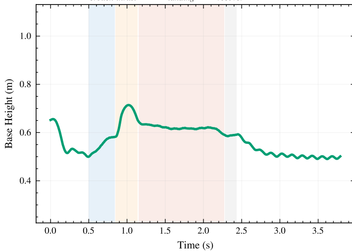
(c) PPO+VMC
