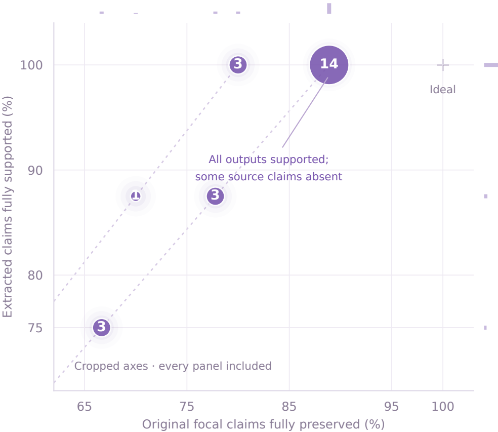
a Coverage × faithfulness
