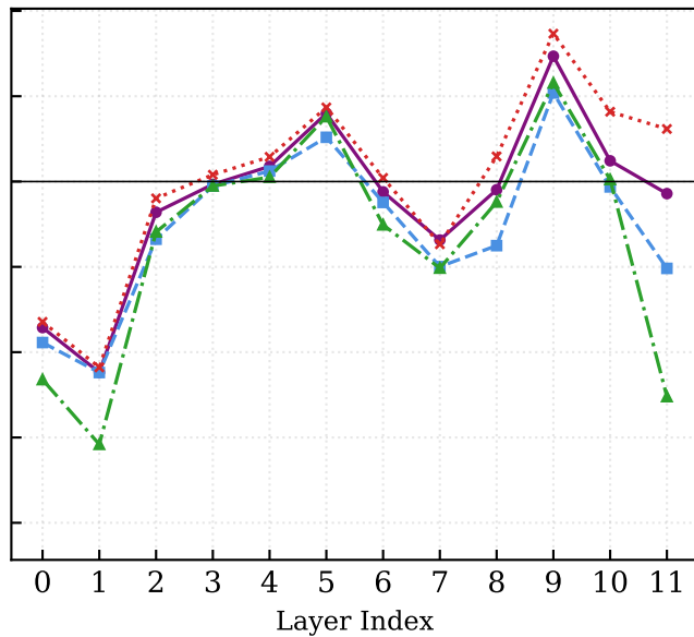
MRPC (Semantic)
