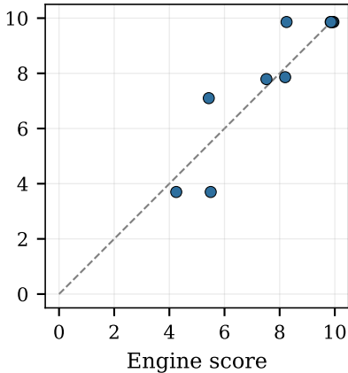
Complexity ( \rho = 0.91 )
