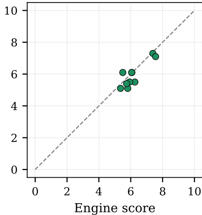
Maintainability ( \rho = 0.71 )
