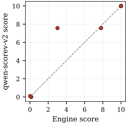
Security ( \rho = 0.98 )
