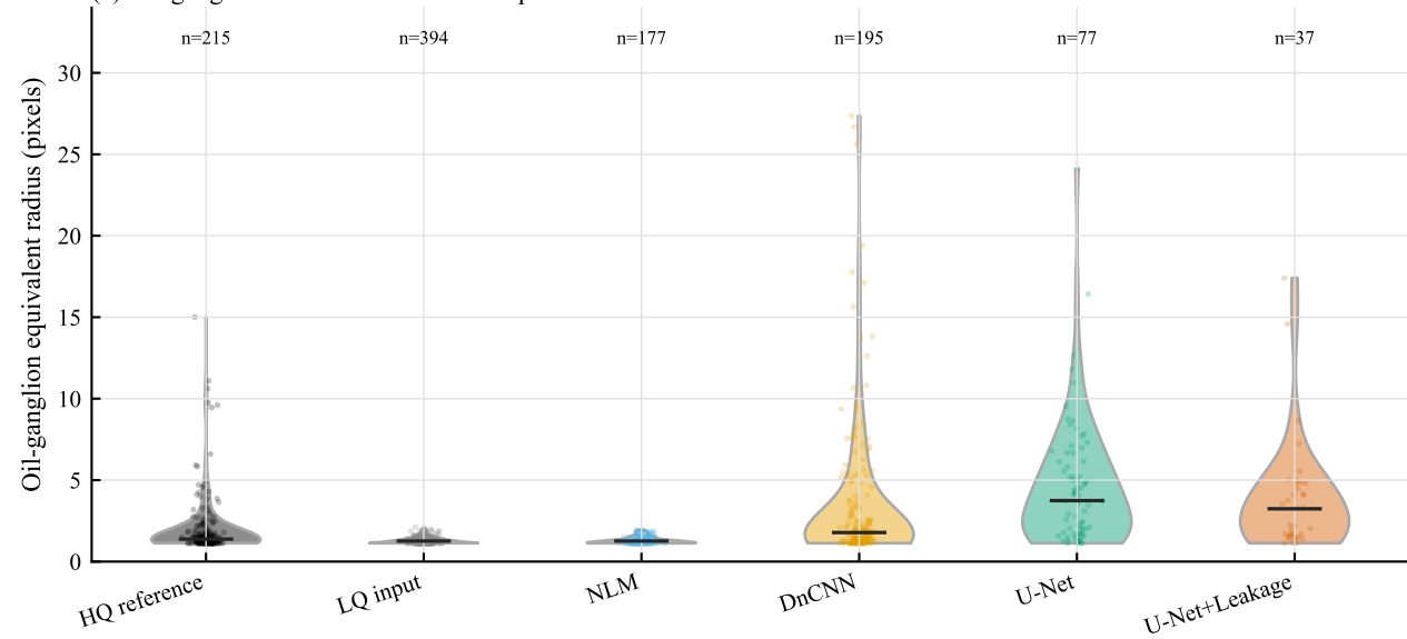
(a) Oil-ganglion size distributions for representative slice 92
