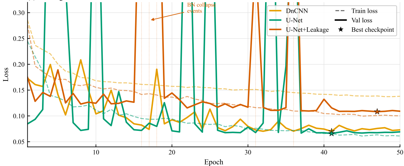
(a) Training and validation loss curves
