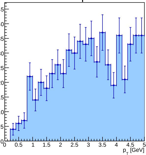
\tau p_T
