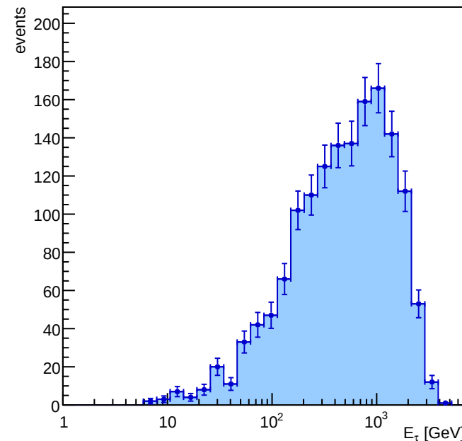
\tau energy
