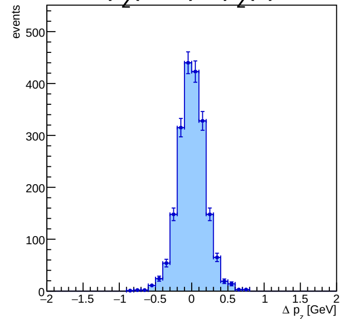
p_z(\text{final}) - p_z(v)
