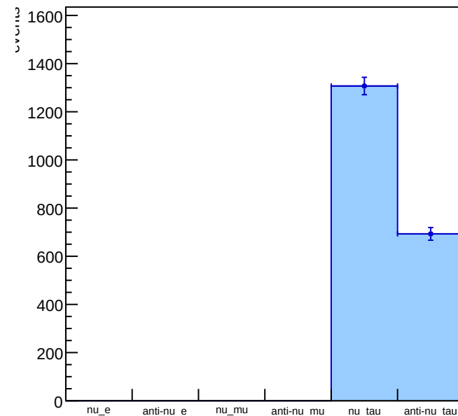
Neutrino flavour
