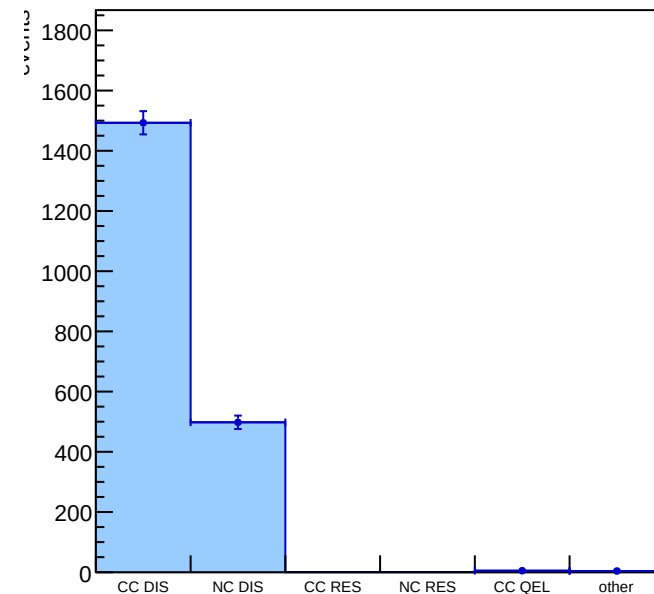
Scattering process
