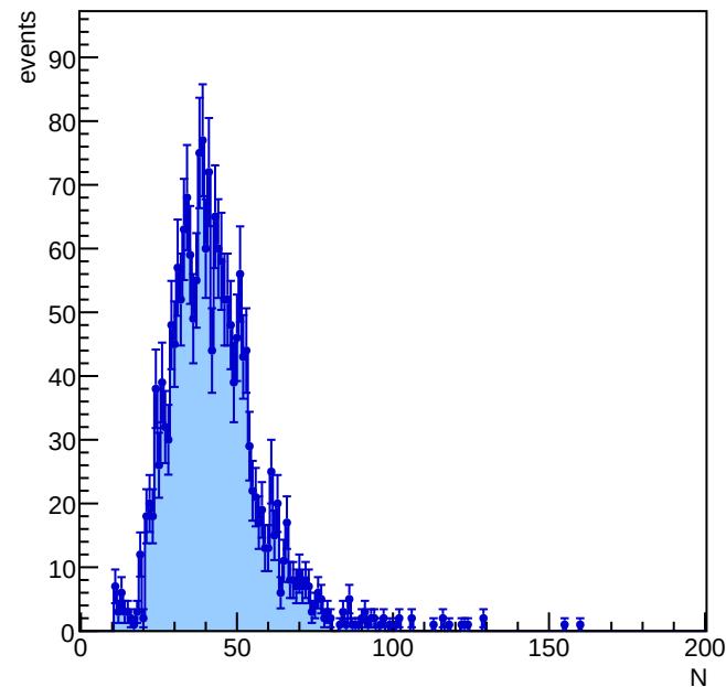
Particles in the event record
