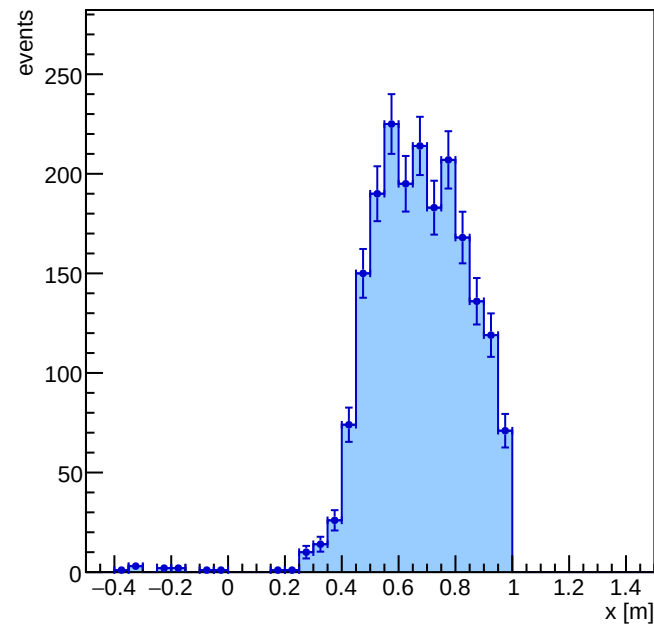
Vertex x
