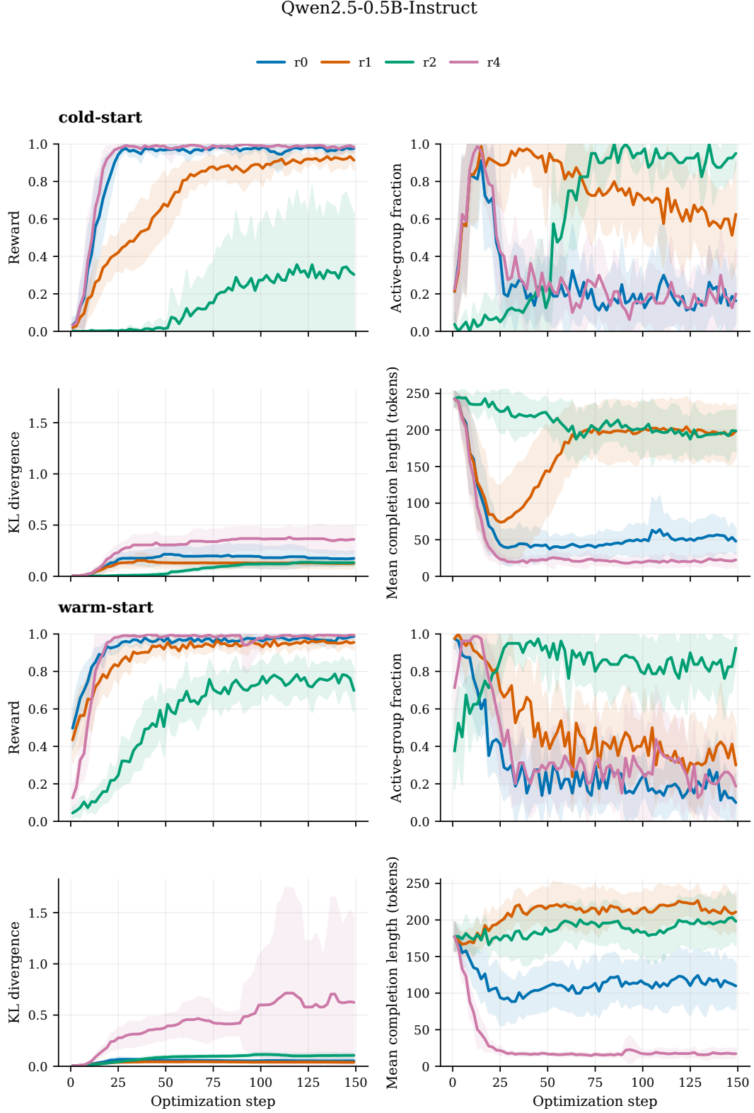
Figure 1: GRPO training diagnostics for Qwen2.5-0.5B.
