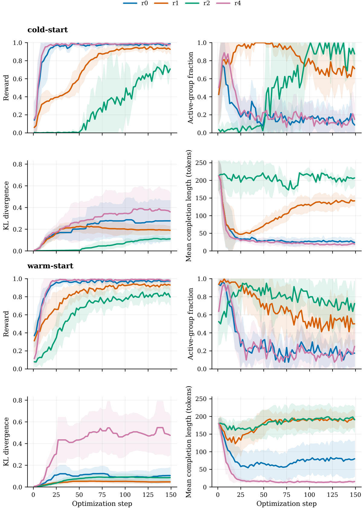
Figure 2: GRPO training diagnostics for Qwen2.5-1.5B. Curves compare reward, active-group fraction, KL divergence, and completion length across reward specifications under original and warm-up SFT initialization.
