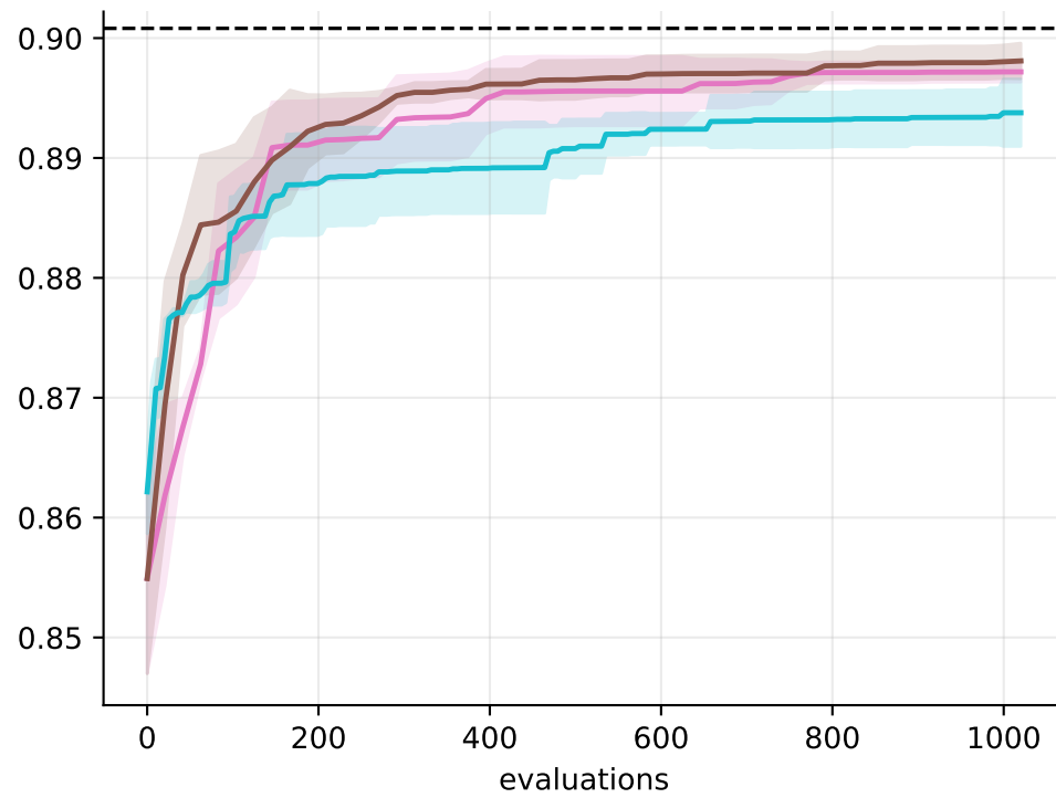
CIFAR-100
