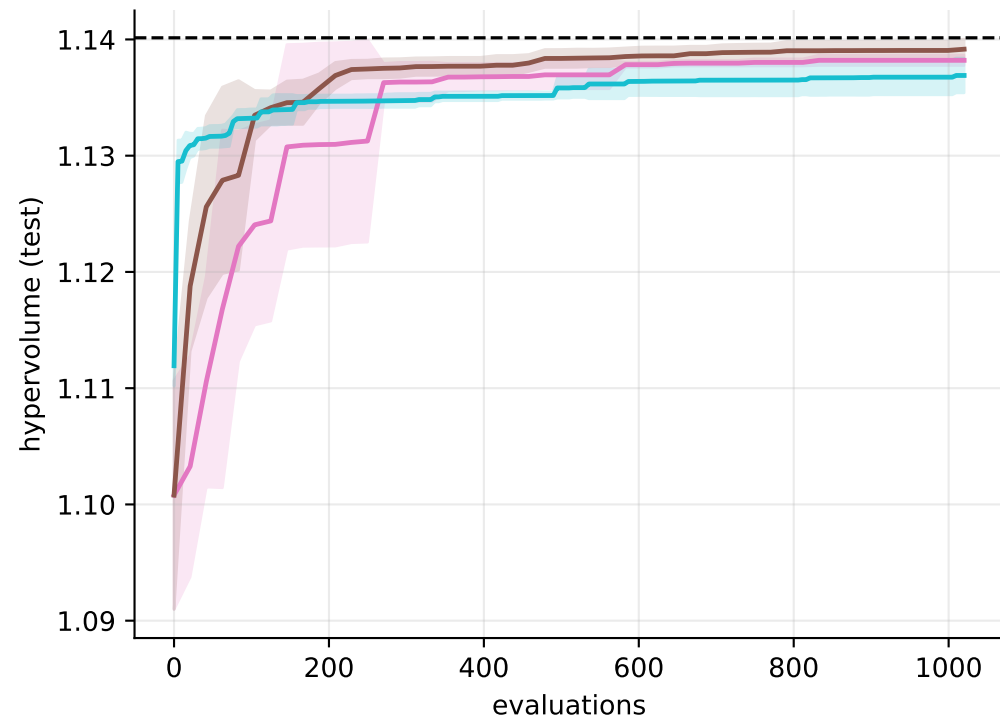
CIFAR-10
