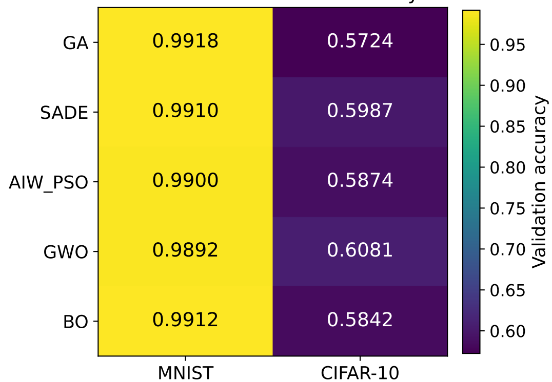
Mean final validation accuracy
