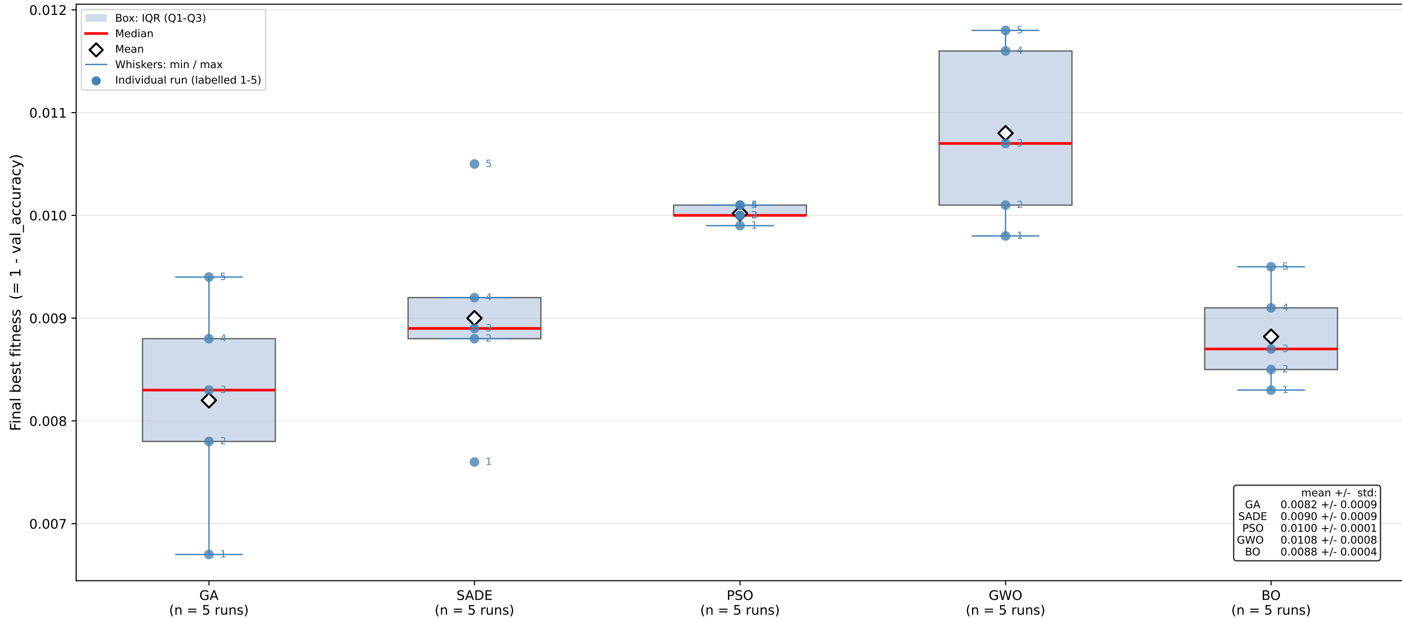
Distribution of the final best fitness across runs - all algorithms
