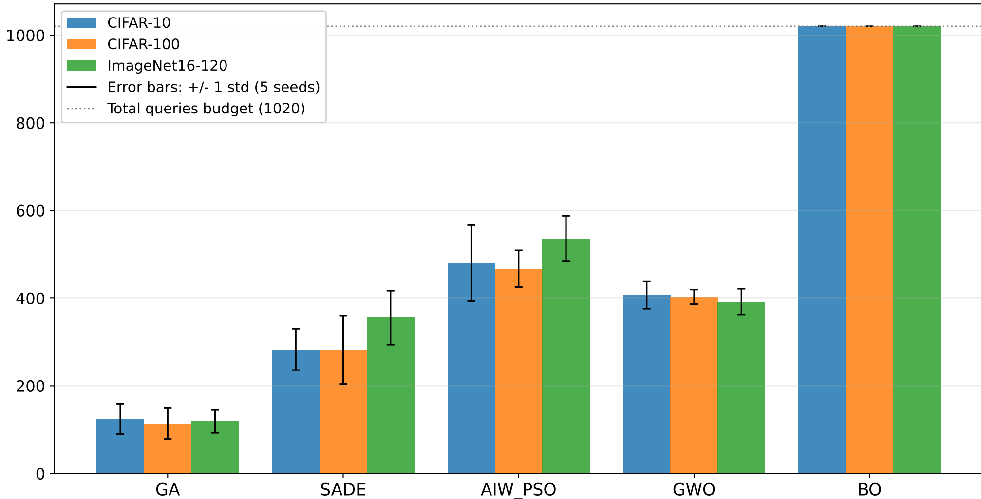
Mean # unique architectures visited per run
