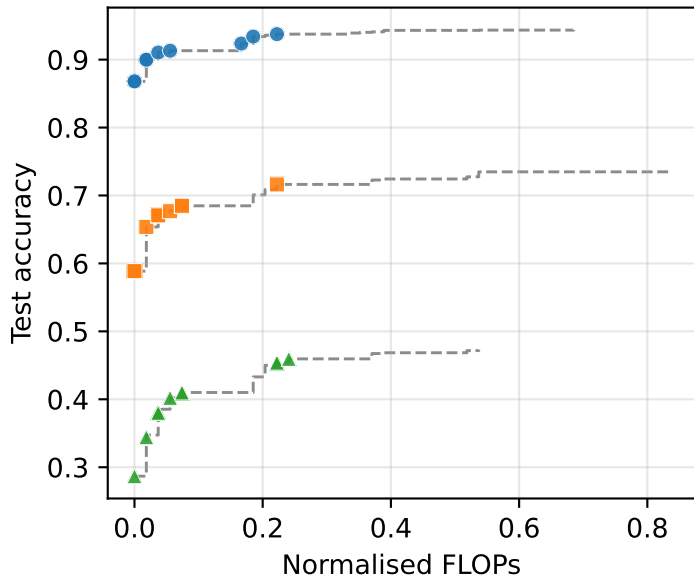
GA
