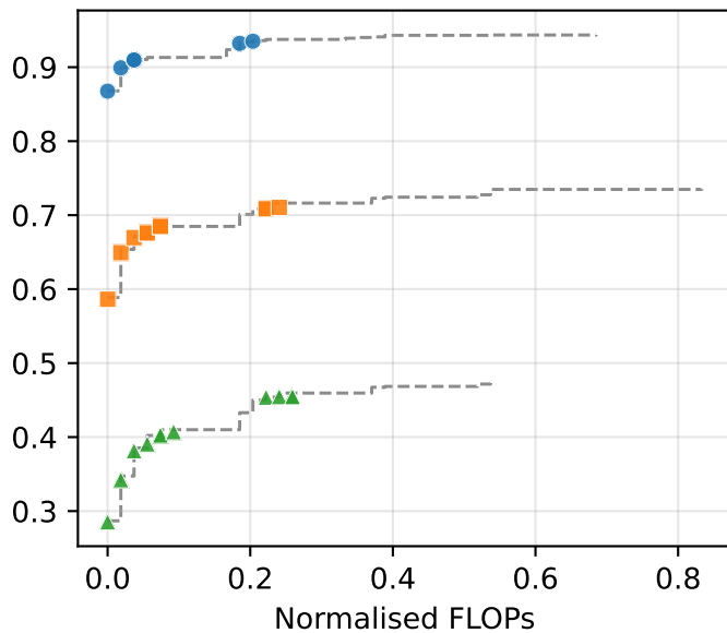
AIW-PSO
