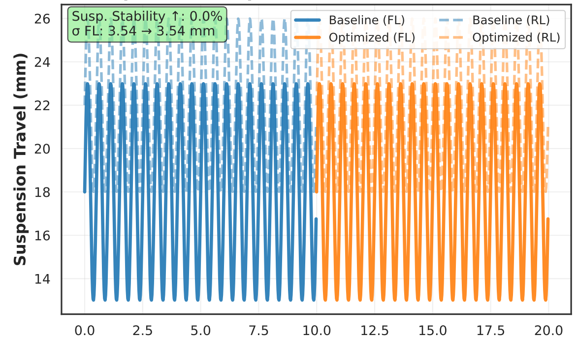
B) Suspension Compression
