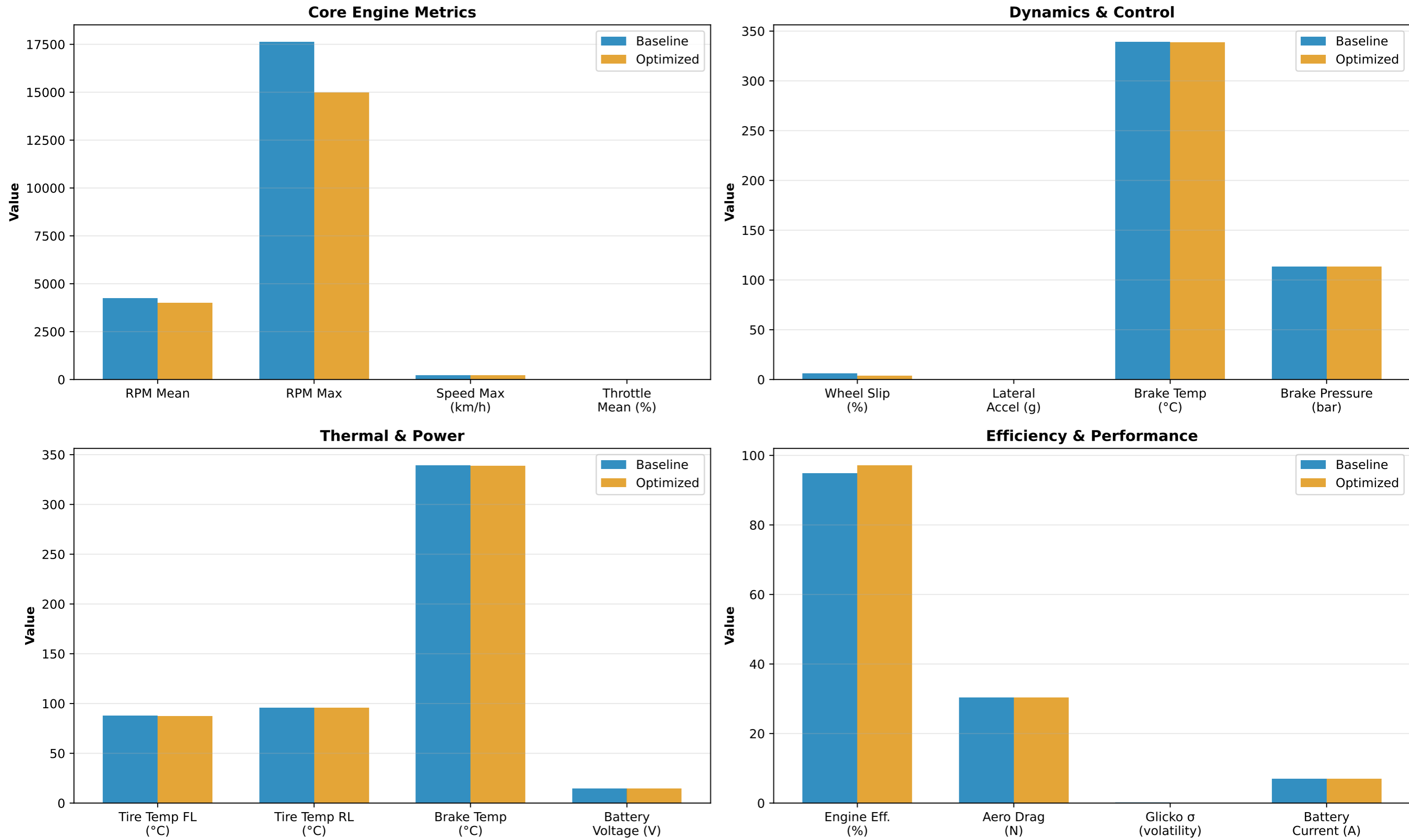
Figure 7: Performance Metrics Comparison with Improvements
