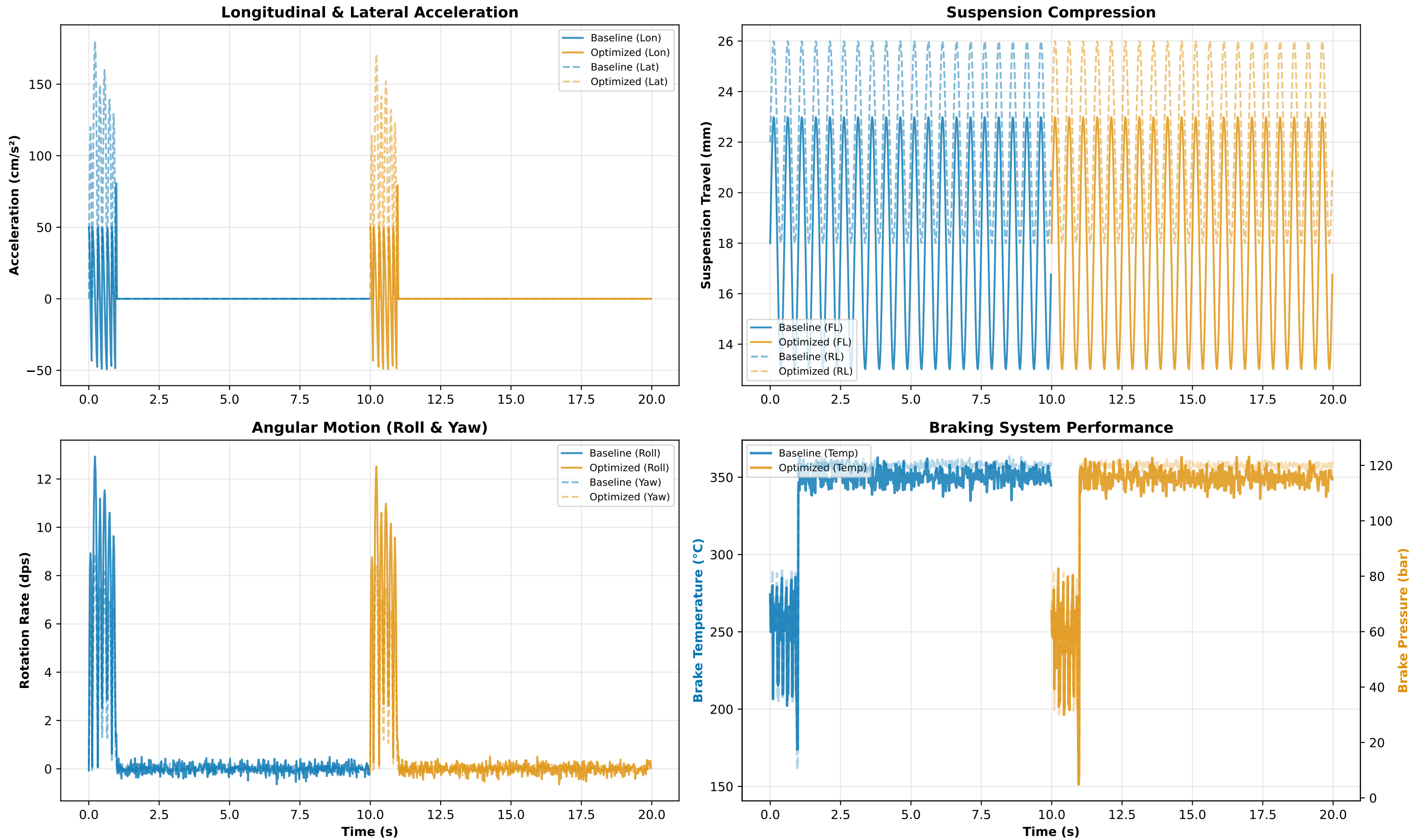
Figure 8: Dynamics, Control & Suspension Analysis
