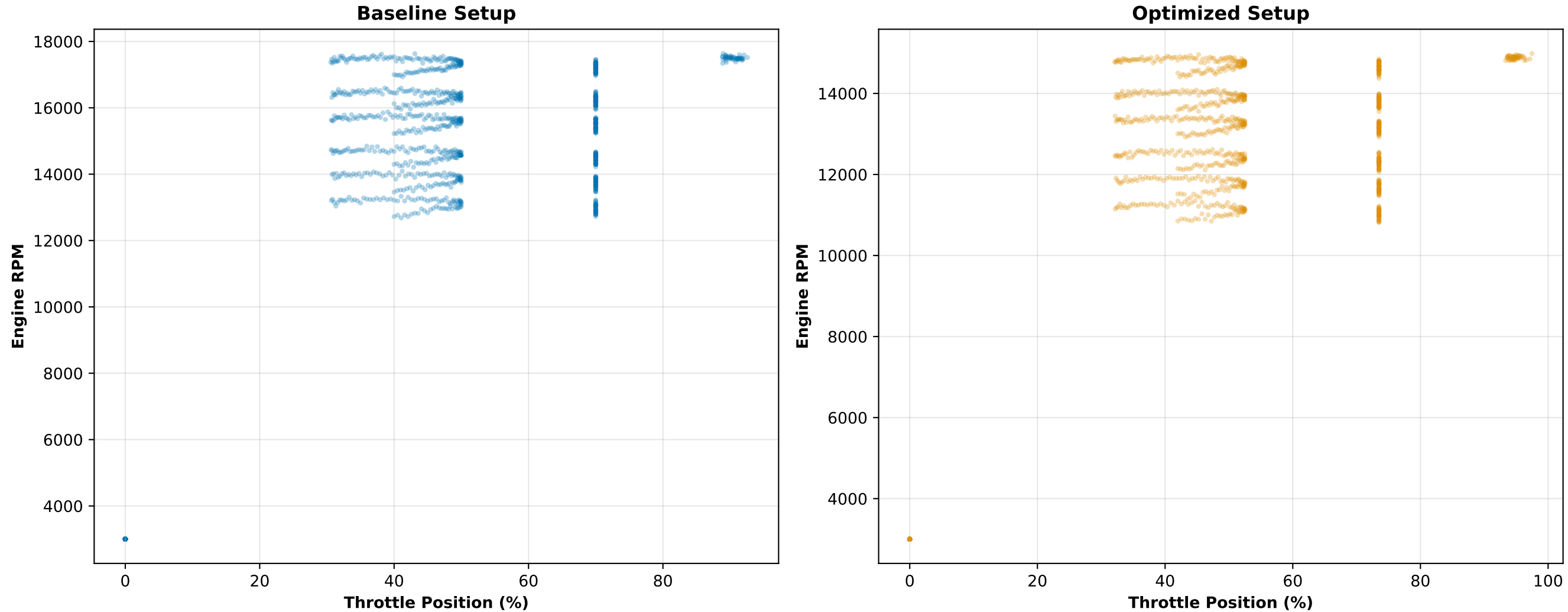
Figure 7: Phase Space Analysis - Throttle vs RPM
