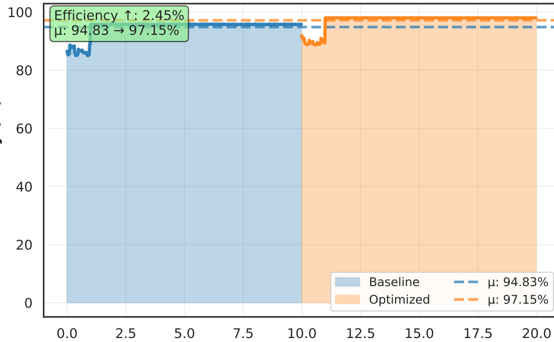
A) Engine Efficiency
