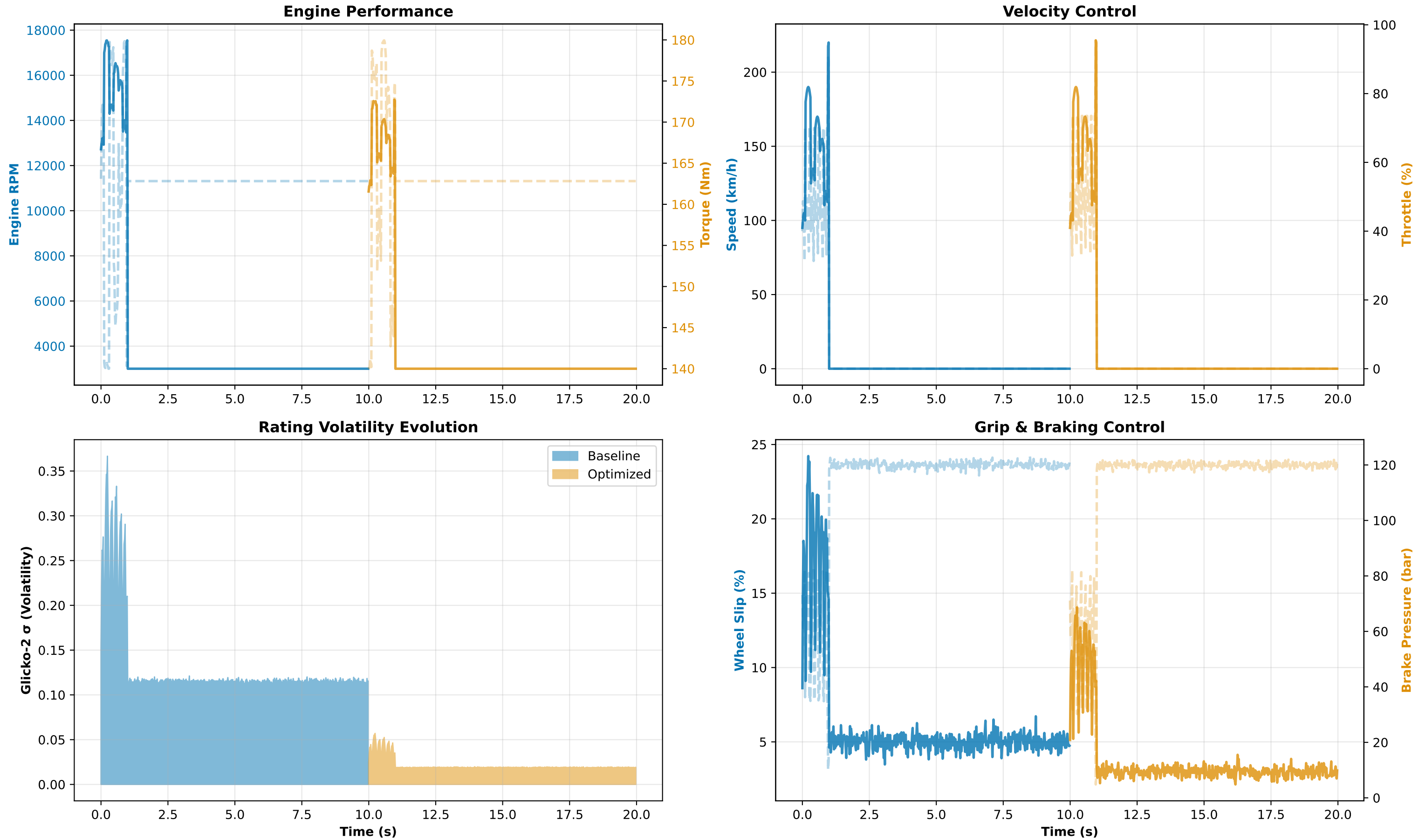
Figure 5: Temporal Evolution - Key Performance Indicators
