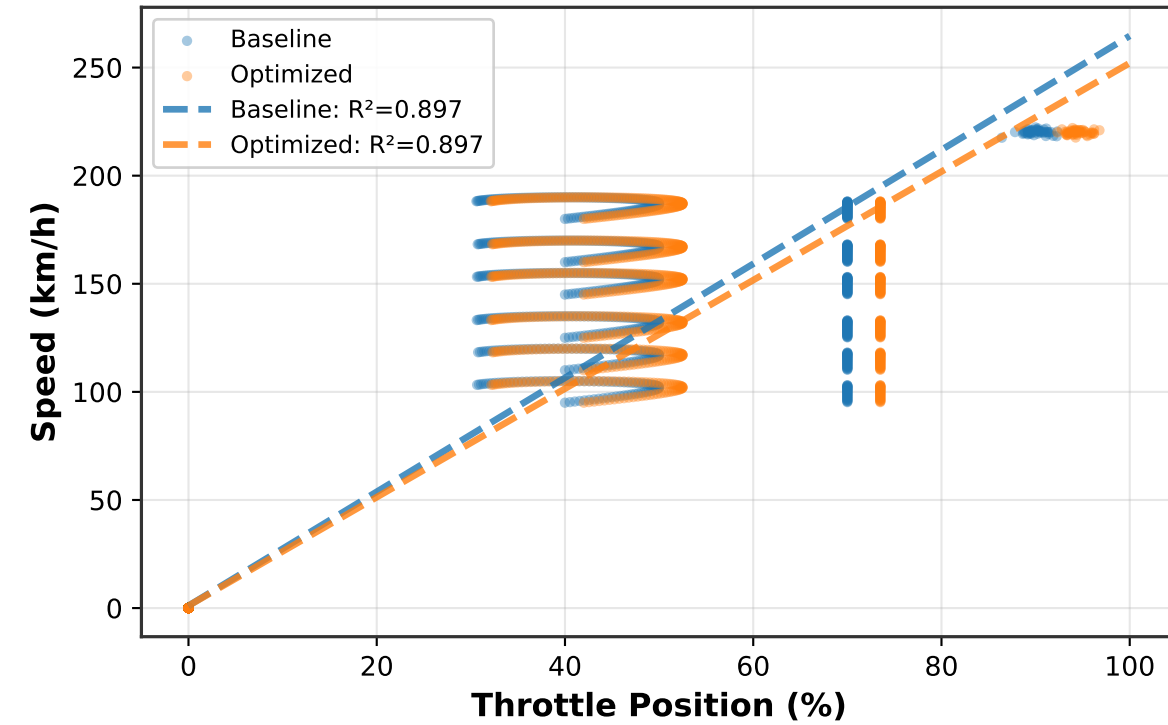
B) Throttle vs Speed Response
