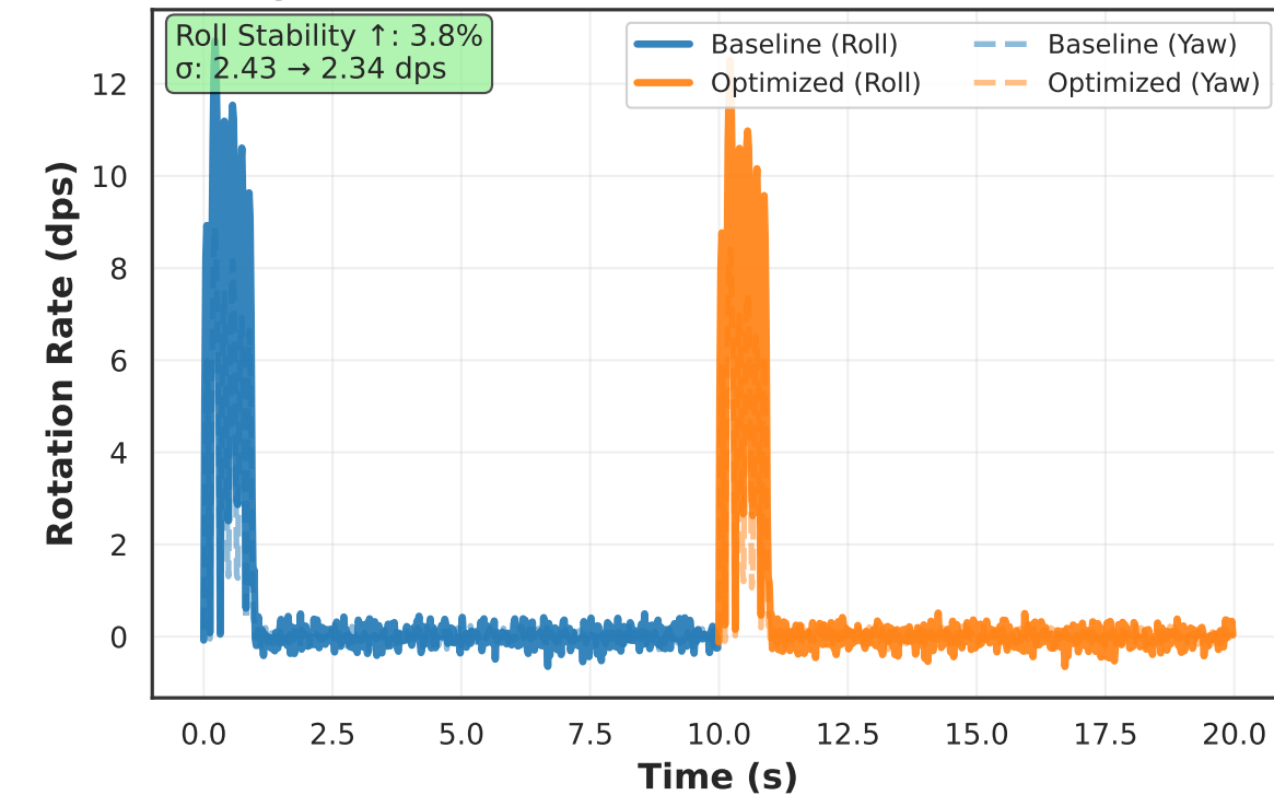
C) Angular Motion (Roll & Yaw)
