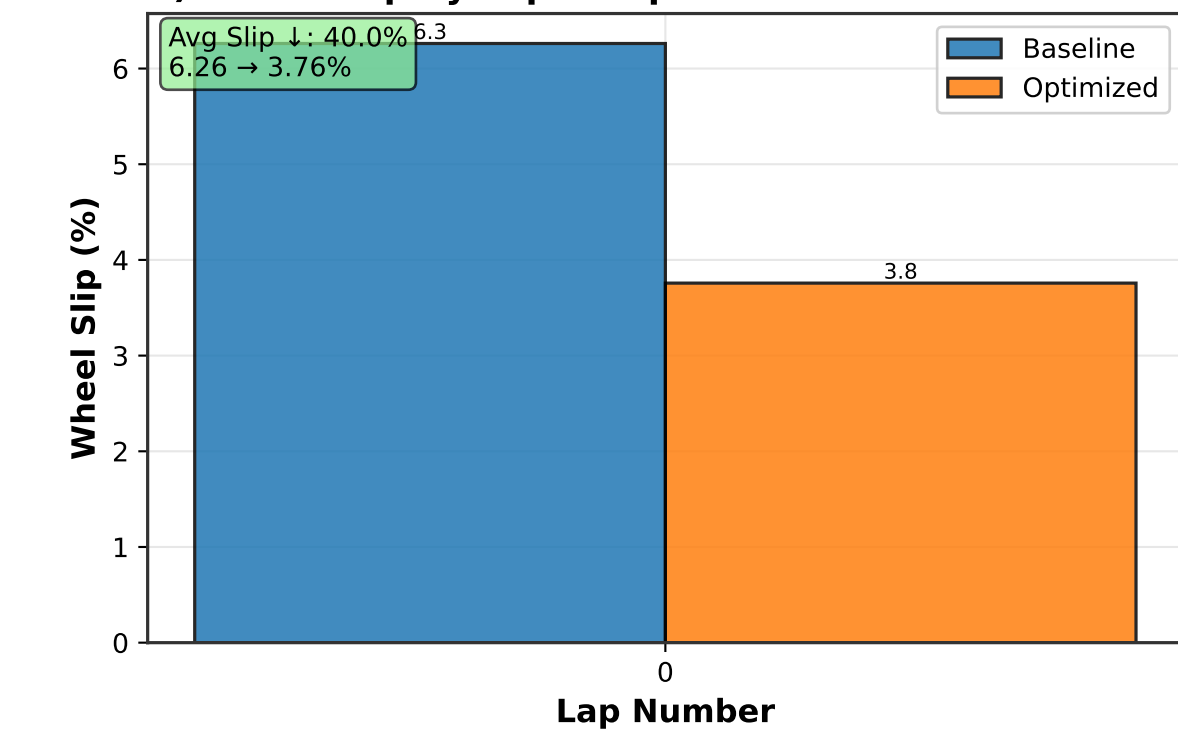
C) Wheel Slip by Lap Comparison
