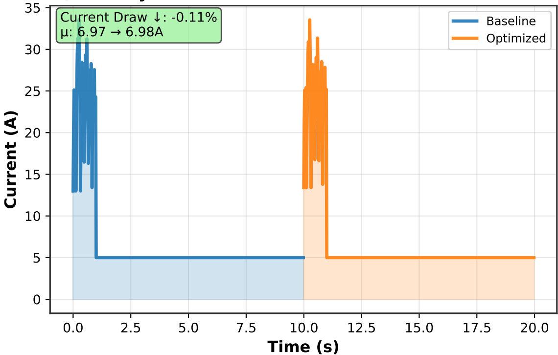
D) Battery Current Draw
