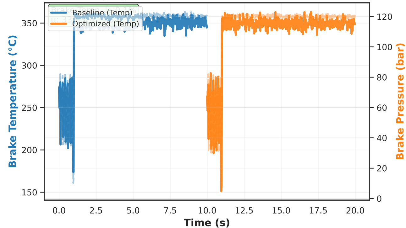
D) Braking System Performance
