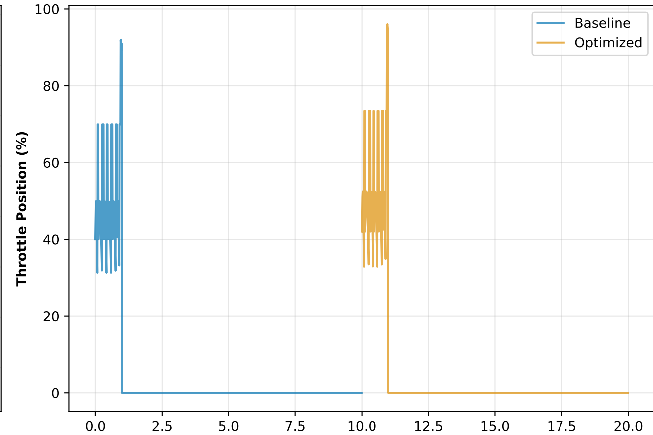
Figure 5: Temporal Evolution - Jerez v4.0 MEGA Dataset
