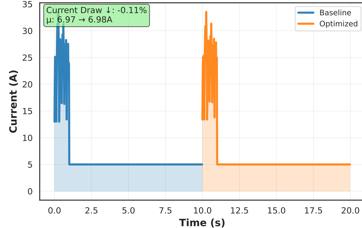
D) Battery Current Draw
