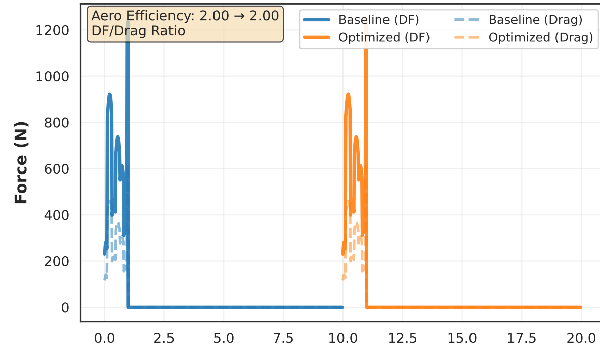
B) Aerodynamic Forces
