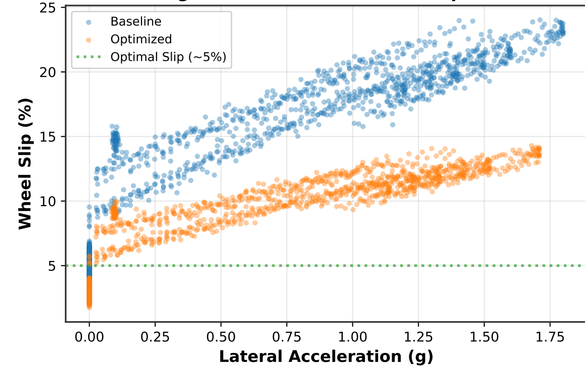
C) Cornering Behavior: Lat. Accel vs Slip
