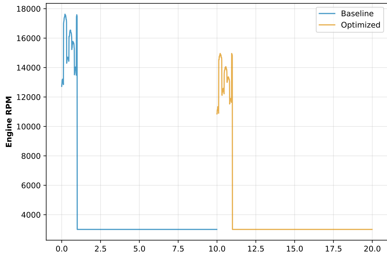
Figure 5: Temporal Evolution - Jerez v4.0 MEGA Dataset
