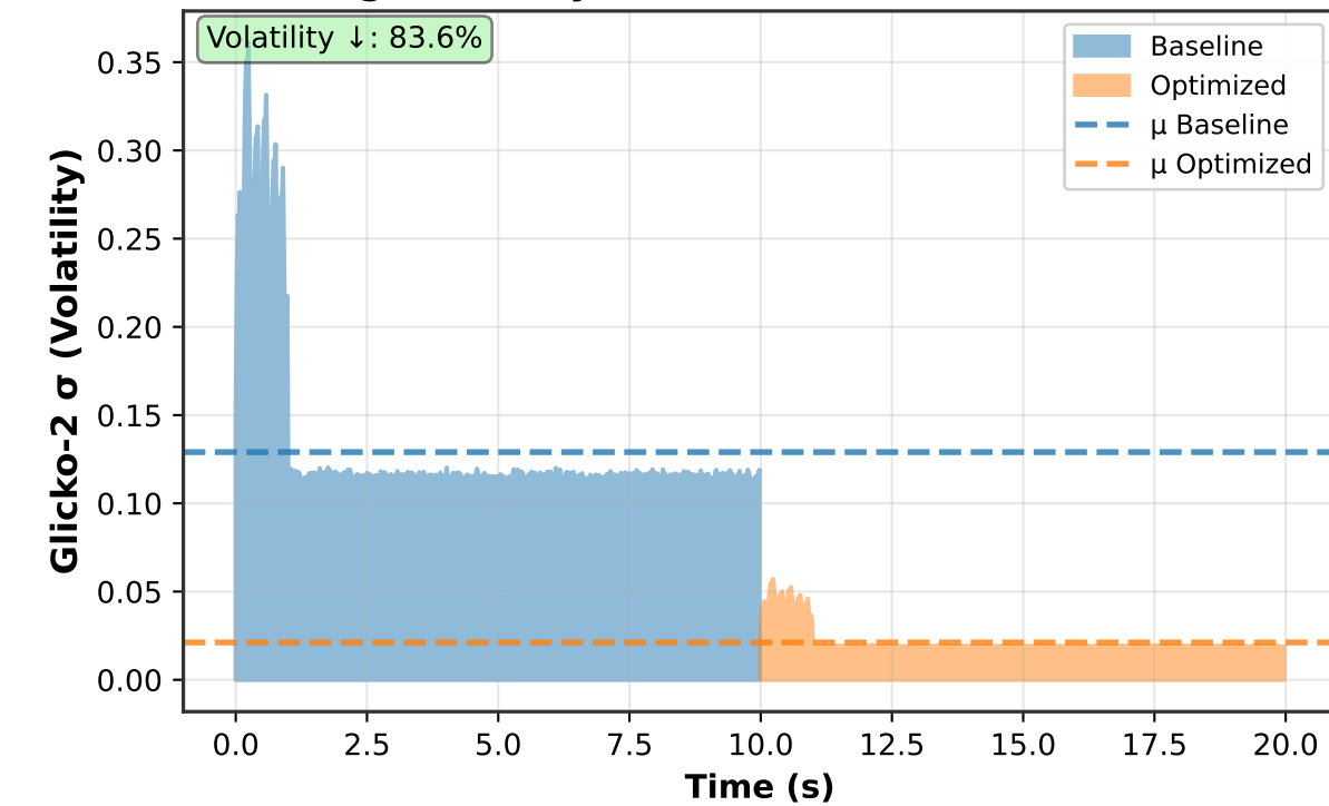
C) Rating Volatility Evolution
