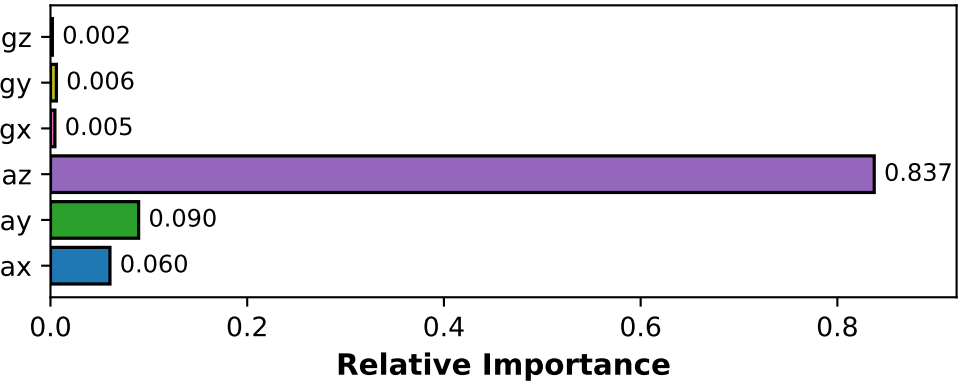
SHAP Feature Importance
