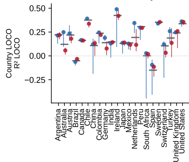
a. Structural BAG Country LOCO
