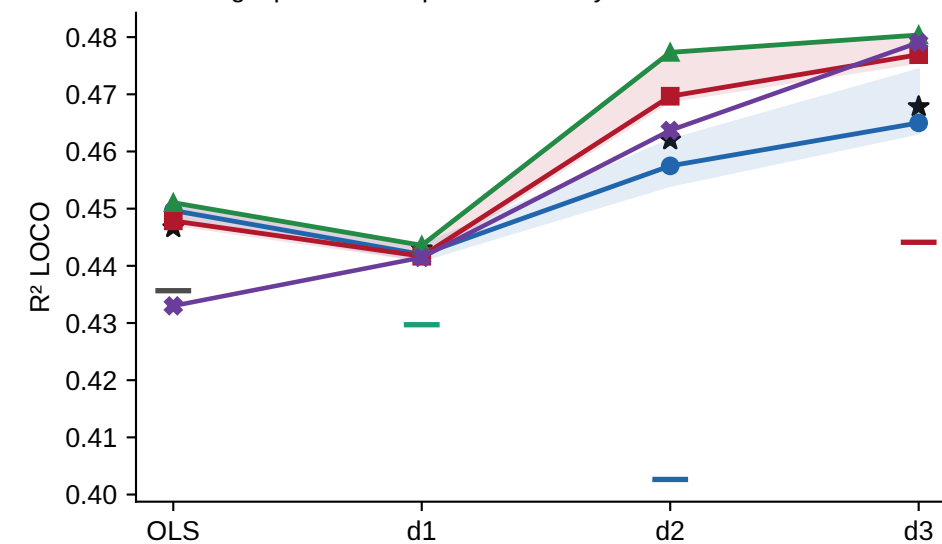
Best single per domain: performance by model level
