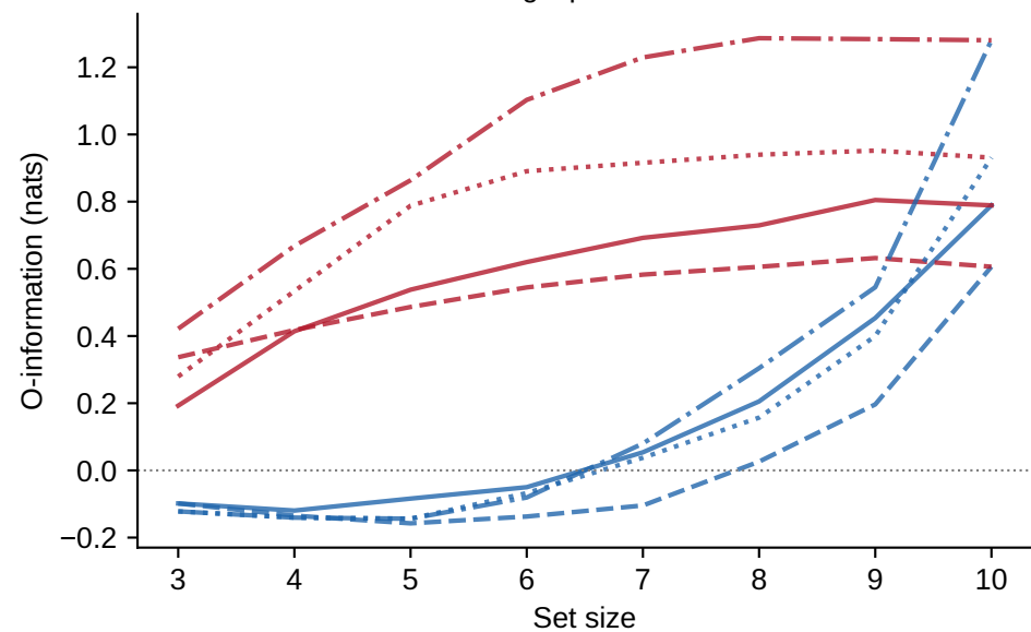
b. Functional BAG — Best single per domain: min/max O-information
