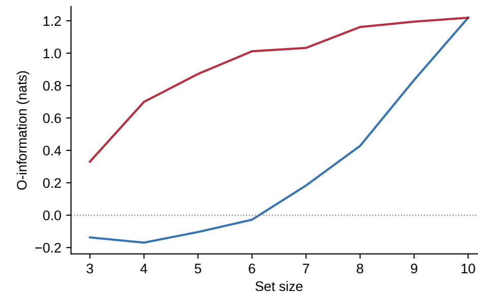
Domain PC1: min/max O-information
