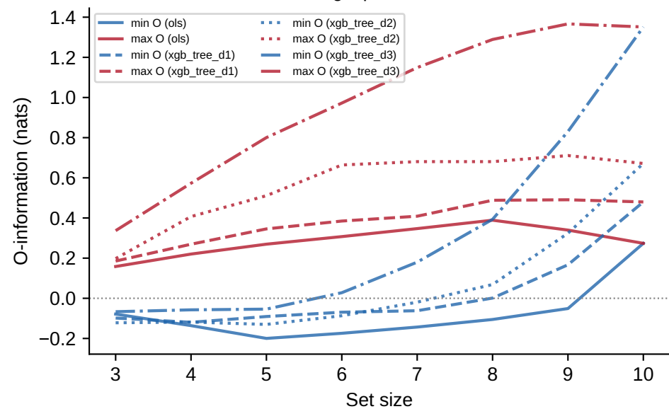
a. Structural BAG — Best single per domain: min/max O-information
