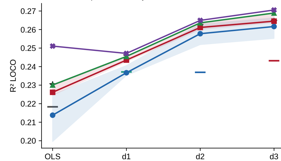
Domain PC1: performance by model level
