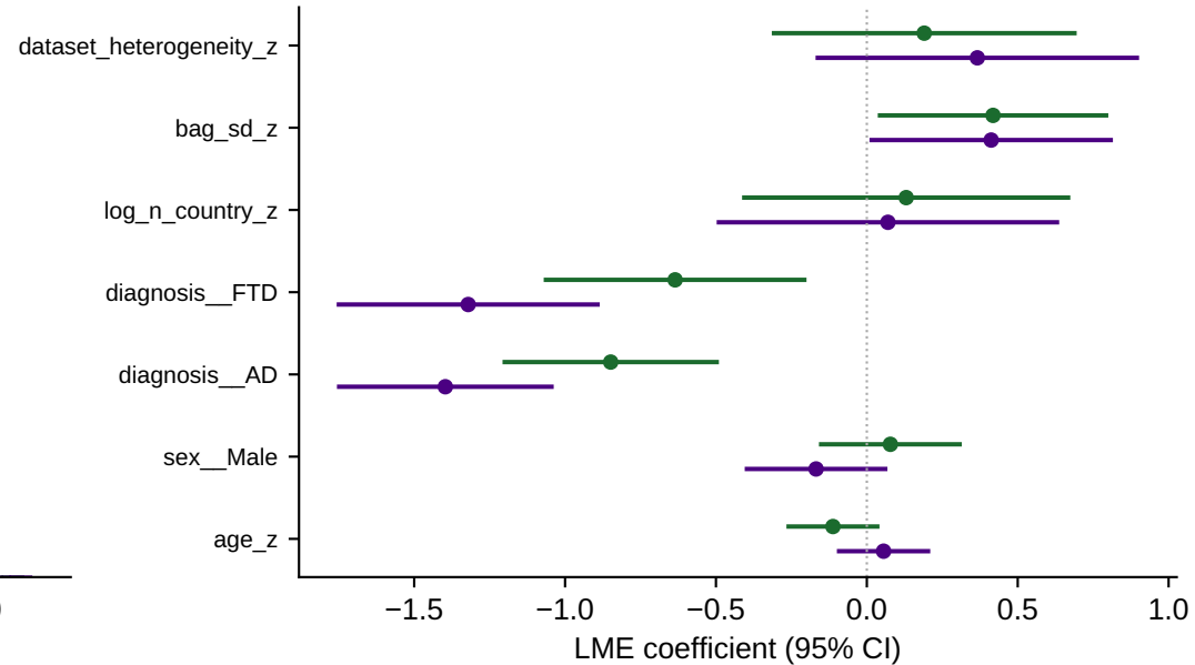
Confound coefficients
