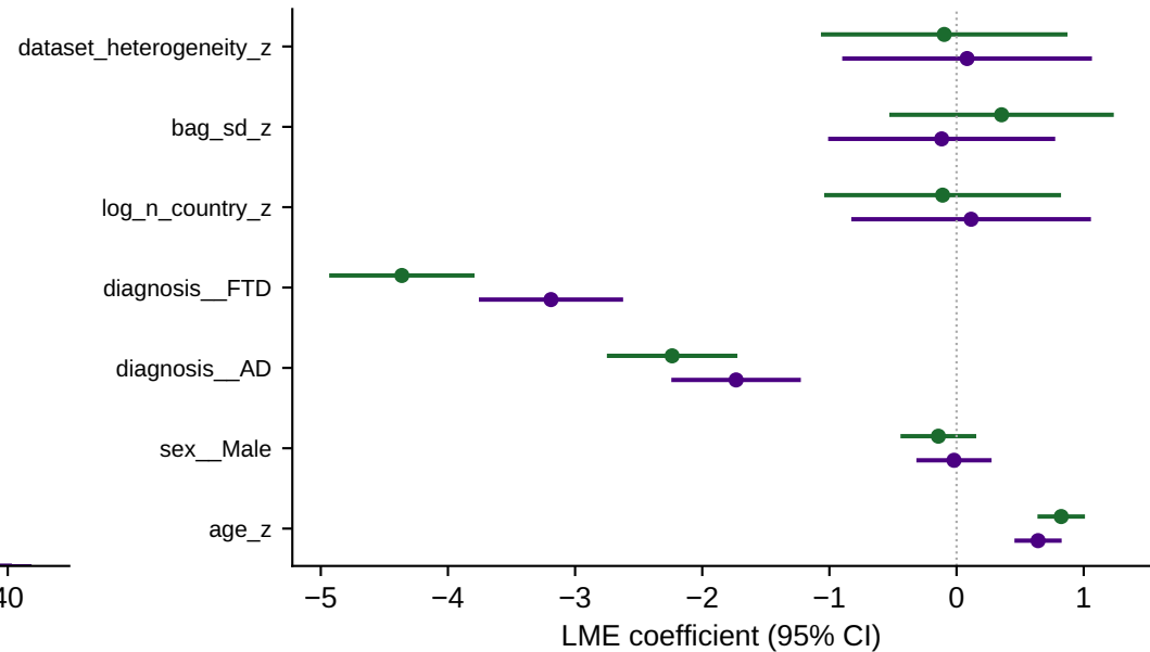
Confound coefficients
