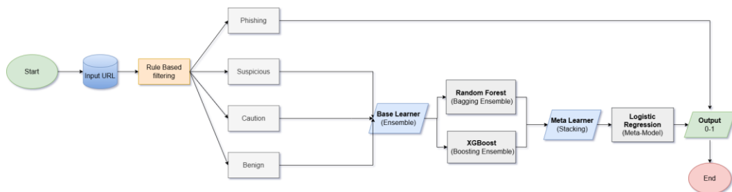
Gambar 4. 11 Rancangan Arsitektur Rule based Filtering
