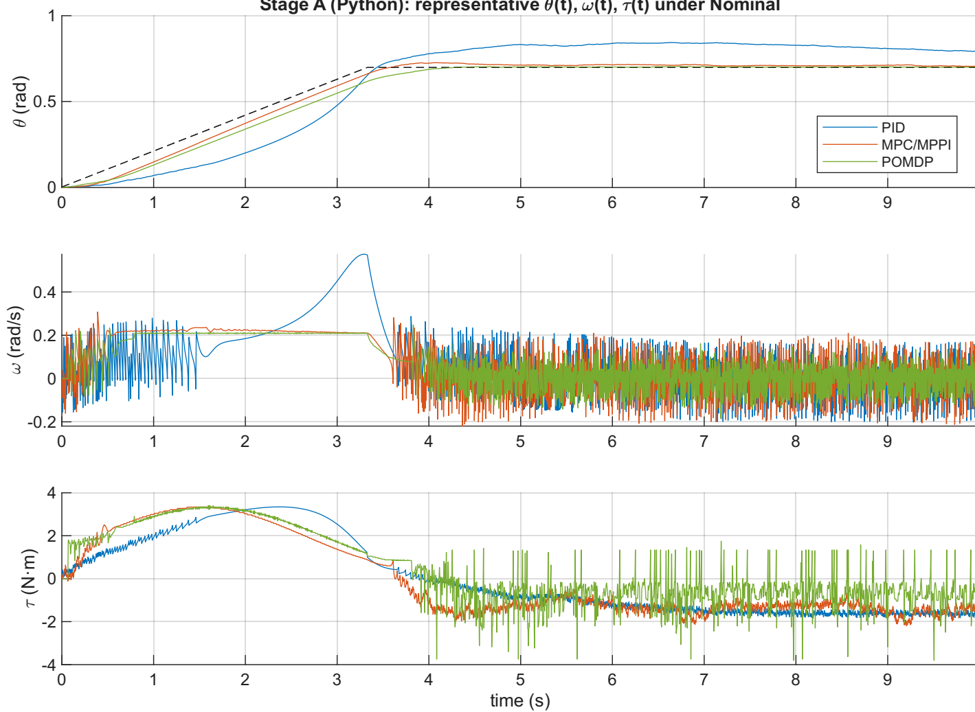
Stage A (Python): representative \theta(t) , \omega(t) , \tau(t) under Nominal
