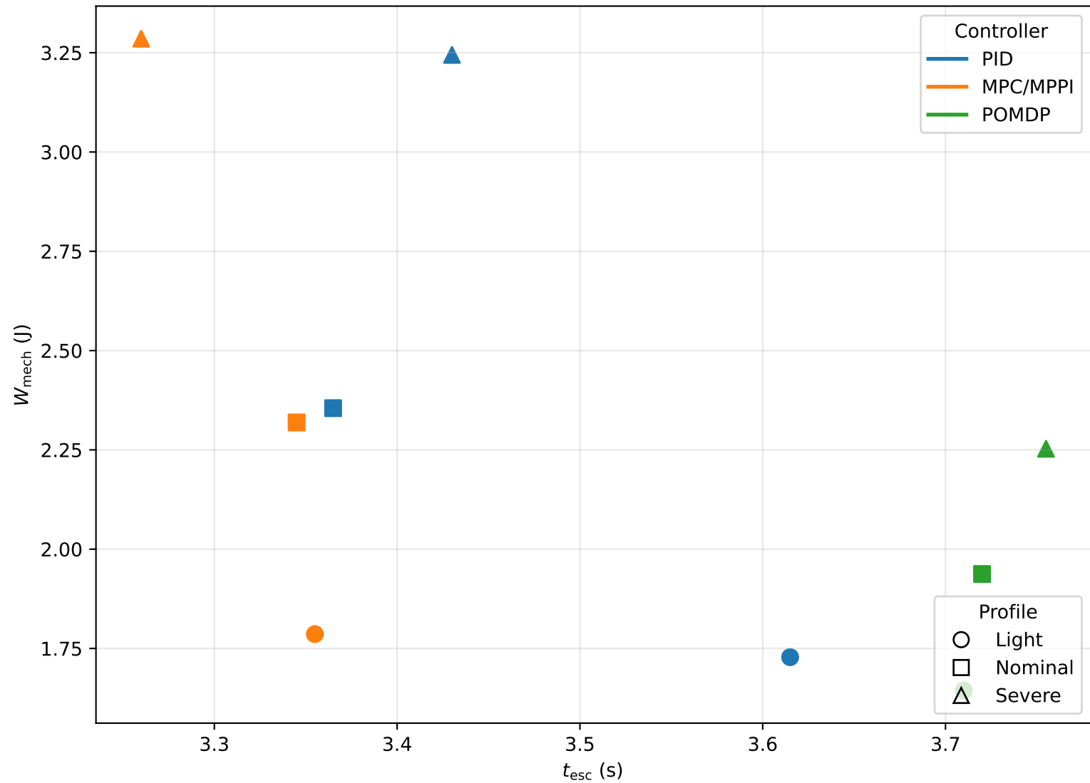
Stage A (Python): time-work trade-off
