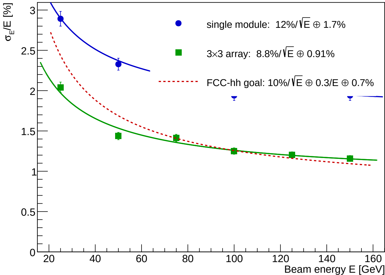
RADiCAL energy resolution: single module vs 3×3 array
