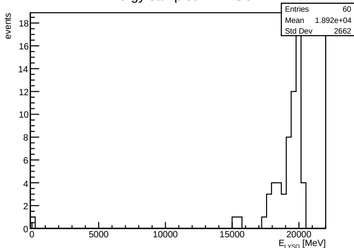
Energy sampled in LYSO
