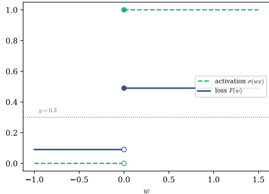
(a) Heaviside: jump discontinuity
