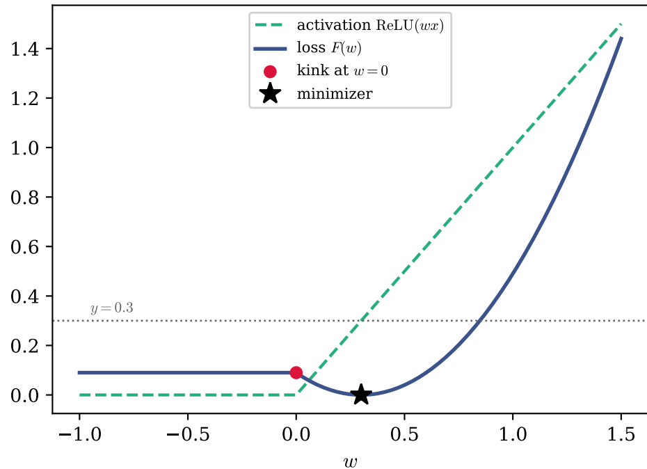
(b) ReLU: non-differentiable kink
