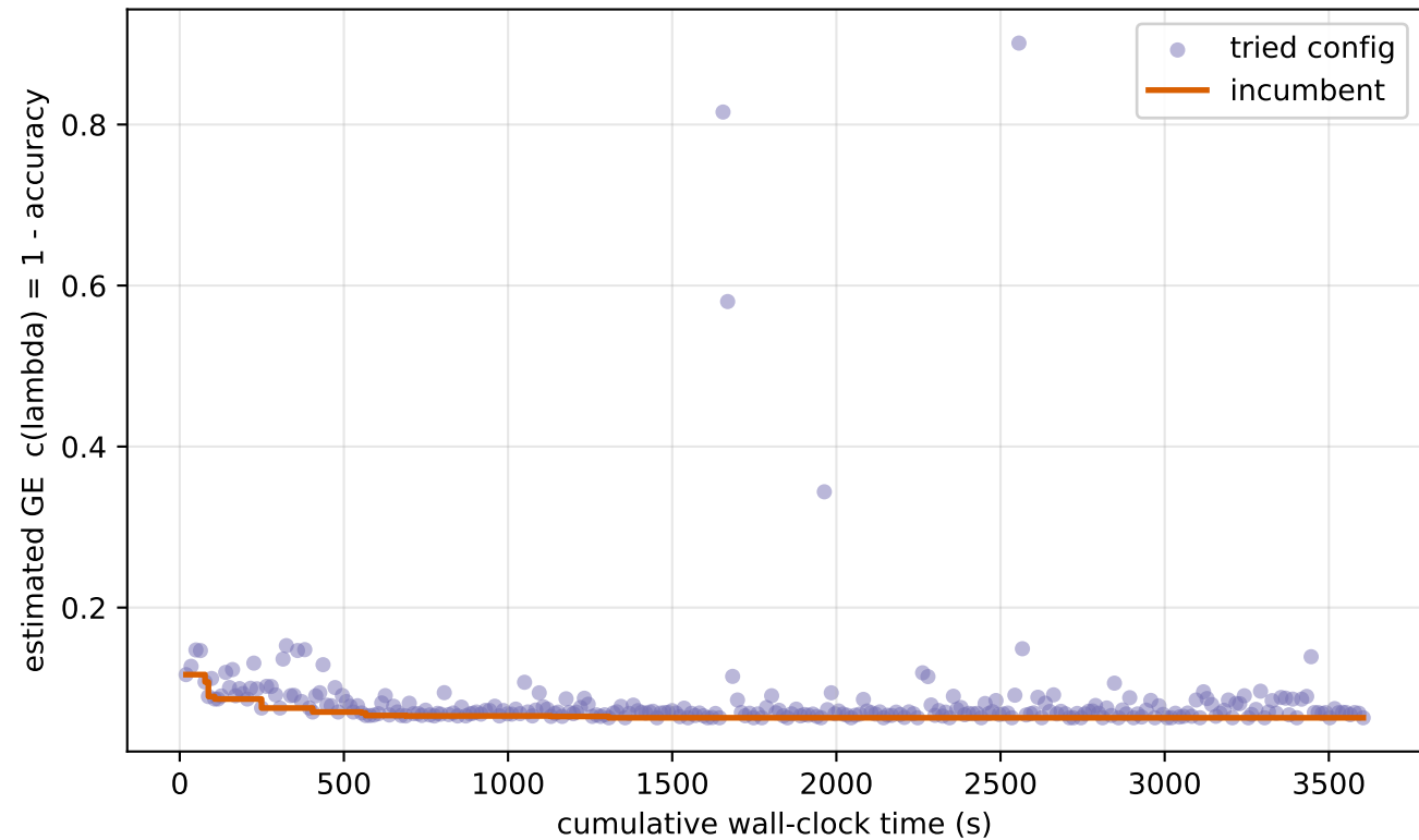
Estimated GE of each tried config: genetic
