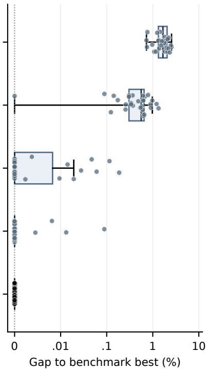
II: medium 30 instances
