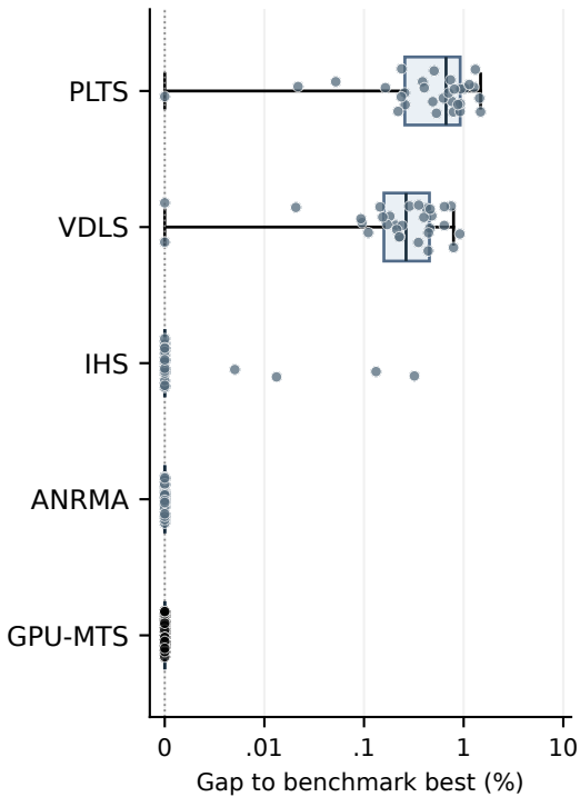
I: small 30 instances
