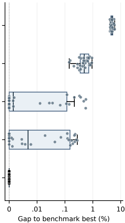
II: large 30 instances
