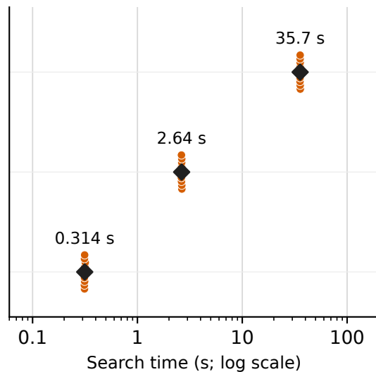
(b) 1300_1300_0.5_2000 512 steps/trajectory · H = 90 s
