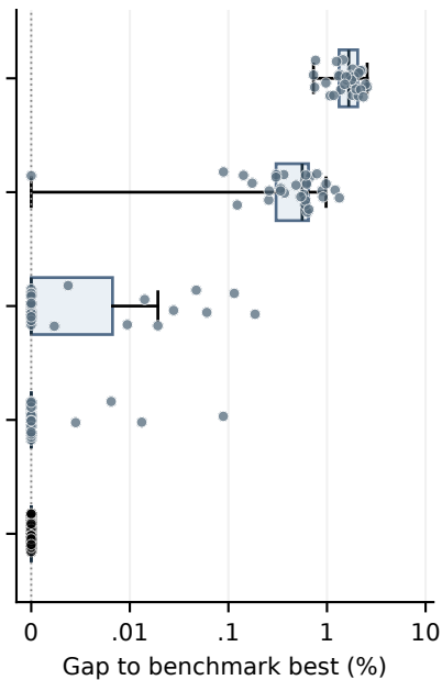
II: medium 30 instances
