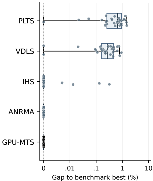
I: small 30 instances
