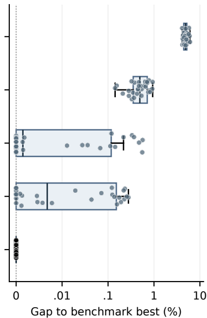
II: large 30 instances
