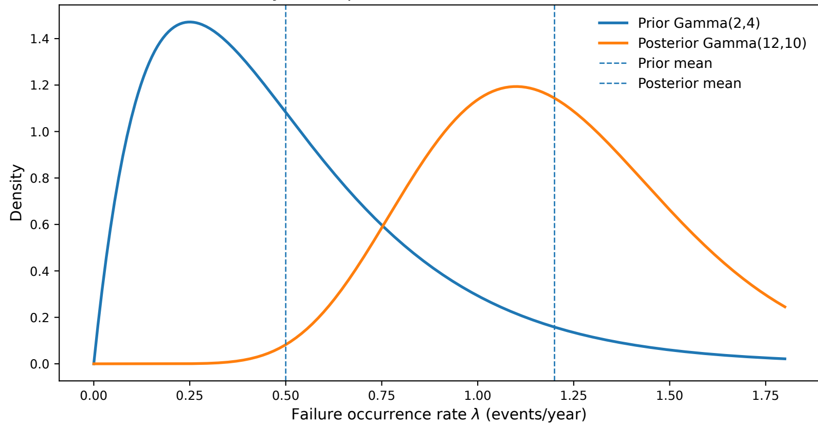
Bayesian update of failure occurrence rate
