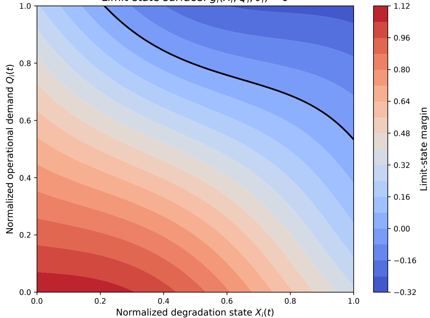
Limit-state surface: g_i(X_i, Q_i, \theta_i) = 0
