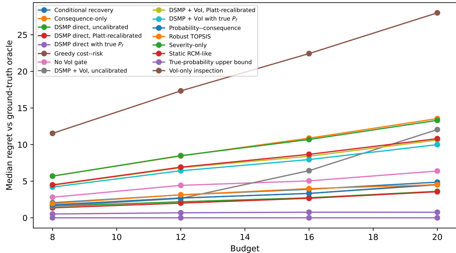
Regret-vs-budget curves
