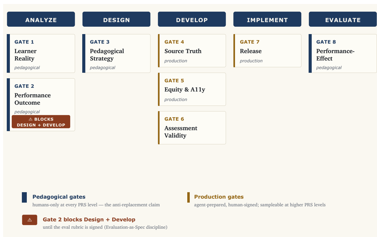
Figure 2 — alt-text caption. The eight AAFL HITL decision gates mapped to ADDIE phases. Gate 1 (Learner Reality, pedagogical) and Gate 2 (Performance Outcome, pedagogical, blocks Design + Develop) sit in the Analyze phase. Gate 3 (Pedagogical Strategy, pedagogical) sits in the Design phase. Gates 4 (Source Truth), 5 (Equity & Accessibility), and 6 (Assessment Validity), all production gates, cluster in the Develop phase. Gate 7 (Release, production) sits in the Implement phase. Gate 8 (Performance-Effect, pedagogical) sits in the Evaluate phase. The four pedagogical gates (1, 2, 3, 8) bookend the framework and remain humans-only at every PRS level. The four production gates (4, 5, 6, 7) cluster in Develop and Implement and are agent-prepared and human-signed, becoming sampleable at higher PRS levels. Gate 2 is marked as the framework's structural blocker: until the eval rubric is signed at Gate 2, neither the Design nor the Develop phase can run.
